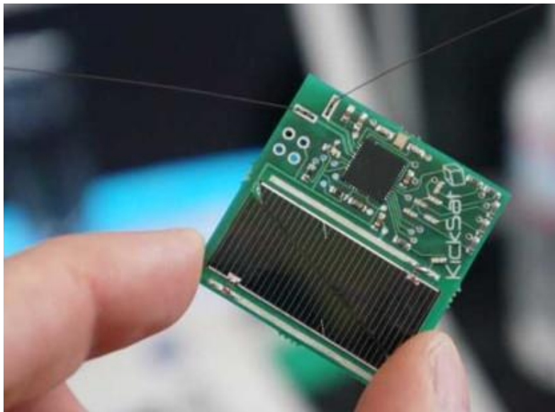
Figure 5. A Sprite spacecraft
