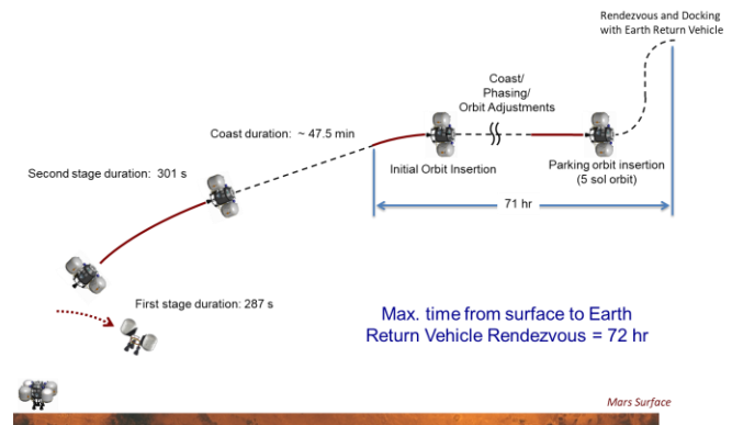
Figure 19. MAV Ascent Trajectory to 5 Sol, Overview
