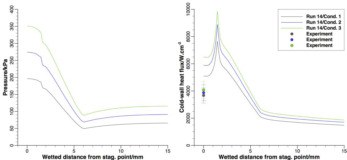
Figure 19: Distributions of surface pressure and heat flux over the nullpoint calorimeter geometry for an arc current of 3000 A and various arc column pressures. The symbols are nullpoint measurements.
