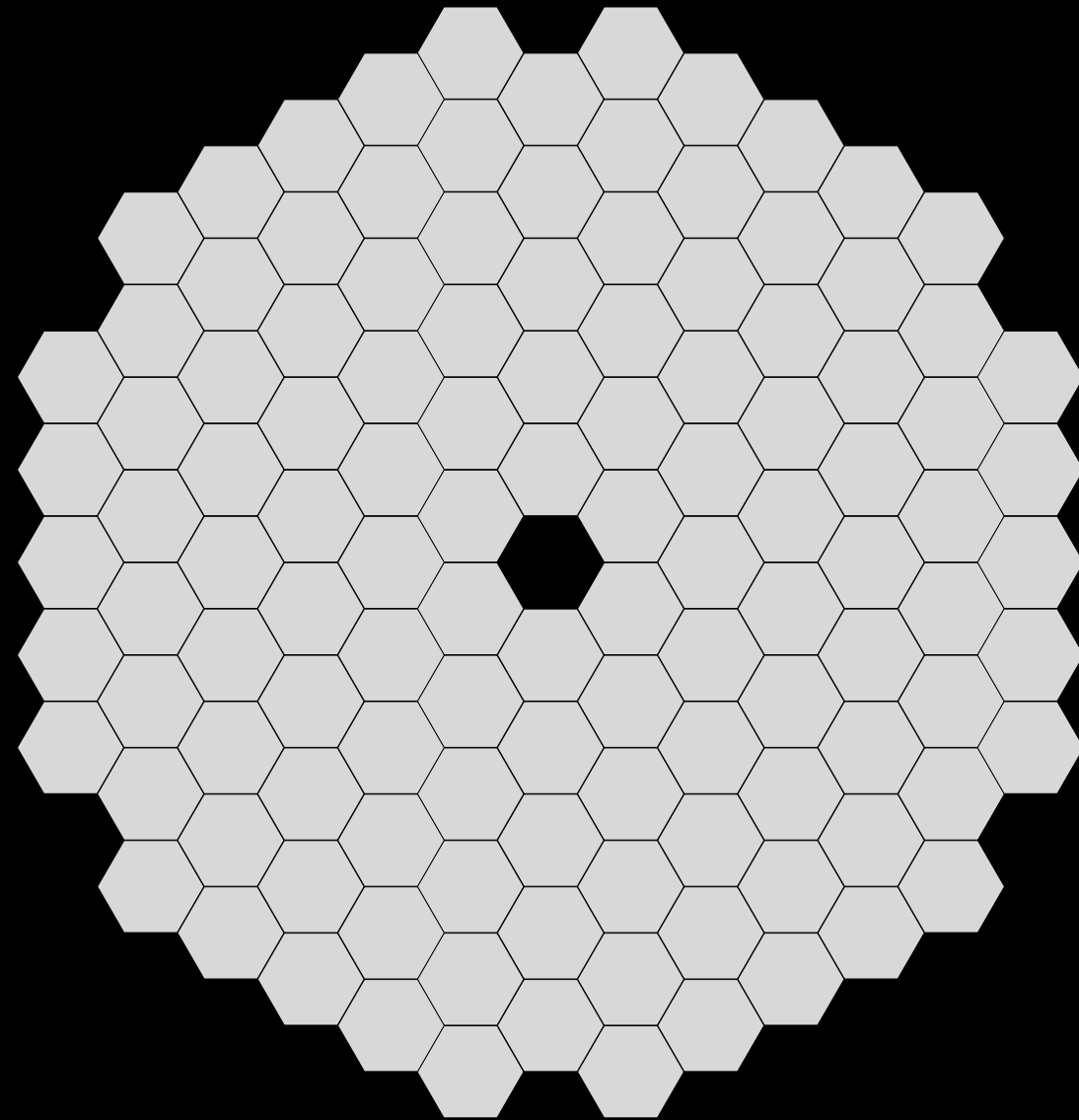
LUVOIR-A 15m Primary Mirror On-Axis Design
