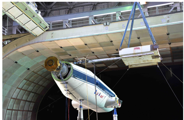
Figure 5. Shake test setup – lateral shaking at forward lifting lug – 0 deg yaw (airplane mode)
