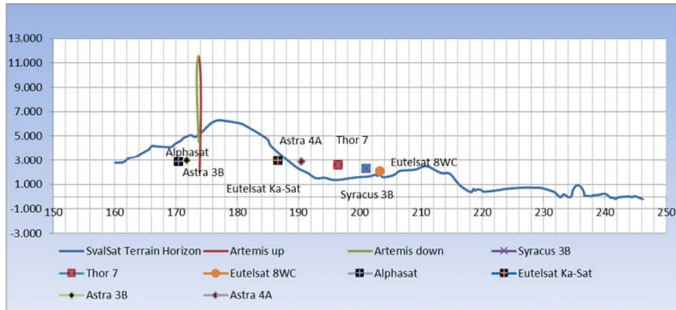
Figure 3. Horizon mask with satellites of opportunity visible from SG61.
