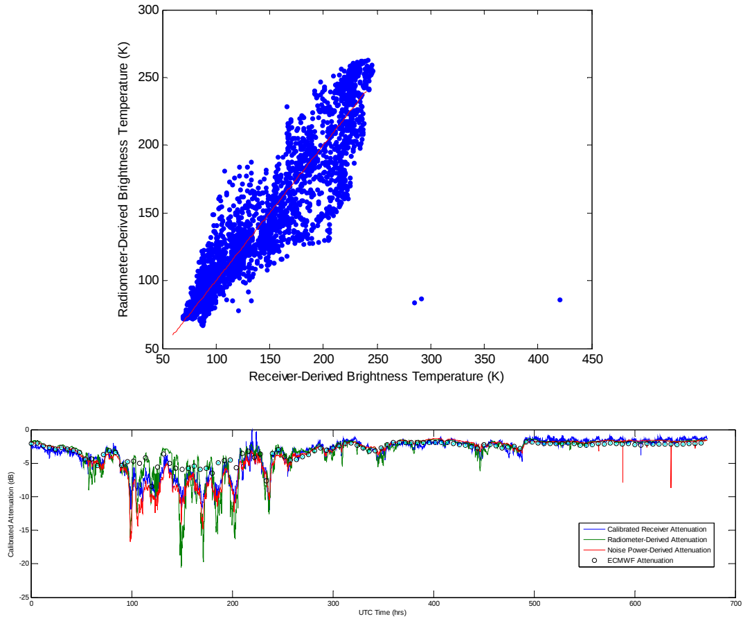
Figure 5. (top) Scatterplot of radiometer-derived brightness temperature at 10 deg elevation angle and noise-power derived brightness temperature (scaled from 2.6 deg to 10 deg) for the month of February 2017. (bottom) Time series comparison of receiver attenuation, radiometer-derived attenuation, noise power-derived attenuation, and ECMWF data for February 2017.
