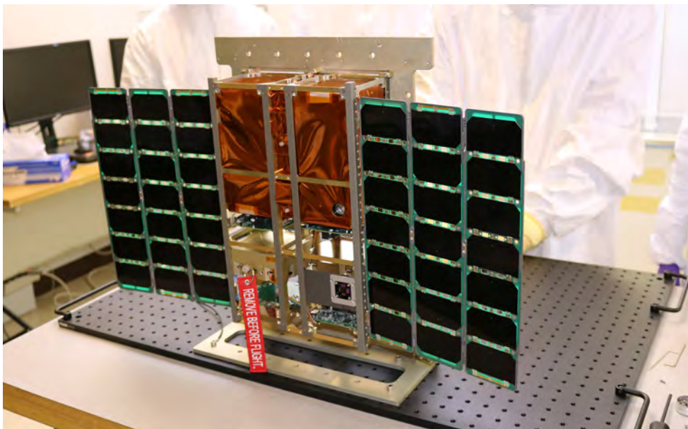
MiniCarb combines NASA's laser heterodyne radiometer (seen in orange) and Livermore's CubeSat Next-Generation Bus, which consists of all the other components. (Photo by Dan Linehan.)
