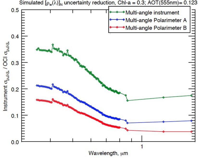
Figure 4. This figure expresses the improvement in retrieved normalized water-leaving reflectance ( [\rho_w(\lambda)]_N ) uncertainty with the use of multi-angle instruments and polarimetrically sensitive multi-angle instruments in addition to OCI. Values are the ratio of tested instrument [\rho_w(\lambda)]_N uncertainty to OCI [\rho_w(\lambda)]_N uncertainty as predicted by a radiative transfer simulation information content analysis (Knobelspiesse et al, 2012, based upon the information theory originally described in Rodgers, 2000).
