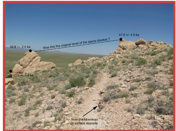
Figure 2. Portion of area mapped near Whale Rock (far left). This area was previously used to ascertain [9,11] an approximate age of the crater (c. 50 ka) and erosion rates (e.g., between 50 and 23 ka, as shown). Although the area is mapped as Kaibab ejecta, it contains blocks of Moenkopi ejecta. From [7].
