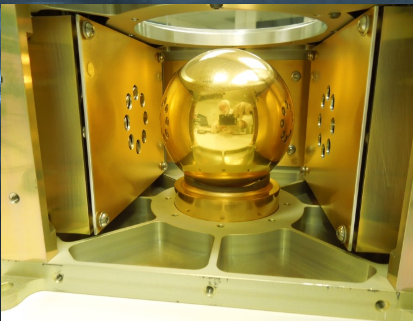
Figure 4. Interior of UV-LED, showing gold-coated proof mass and 2UV-LED boxes on either side
