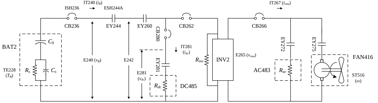
Figure 2. ADAPT-Lite schematic.
