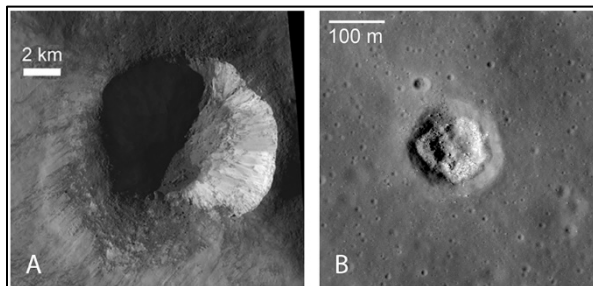
Figure 1. (A) An impact crater formed on the rim of Gibbs crater. Regional slope from top-right to bottom-left is 28^\circ . [ -17.50^\circ S/ 85.18^\circ E] (B) A small impact crater in the lunar mare near the Apollo 12 site showing concentric morphology inferred to be a result of a layer of regolith over a more competent unit. [ -3.297^\circ S/ 336.708^\circ E]
