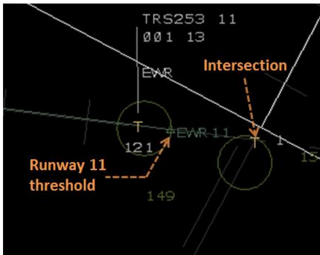
Figure 9. Example of a 14-second STA difference with resulting slot marker location and arrival pair spacing at the runway
