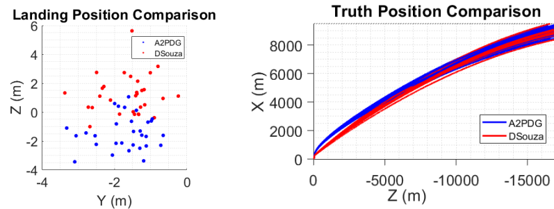
Figure 2: Landing Accuracy Comparison (L), As-flown Trajectory with Navigation Dispersions (R)
