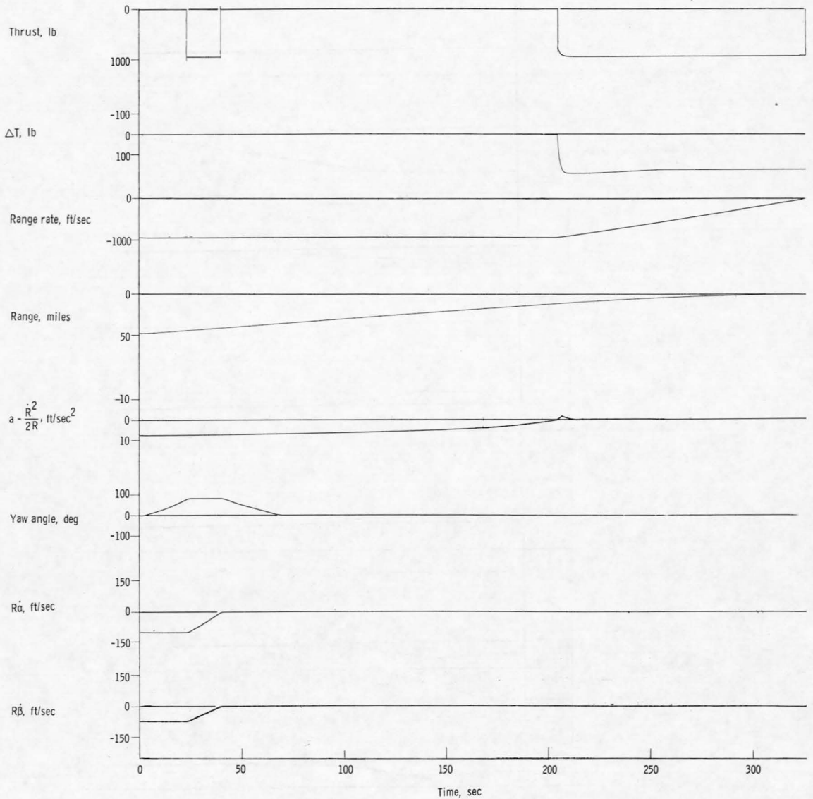
Figure 7.- Time history of the terminal phase of rendezvous for modulated thrust control.
