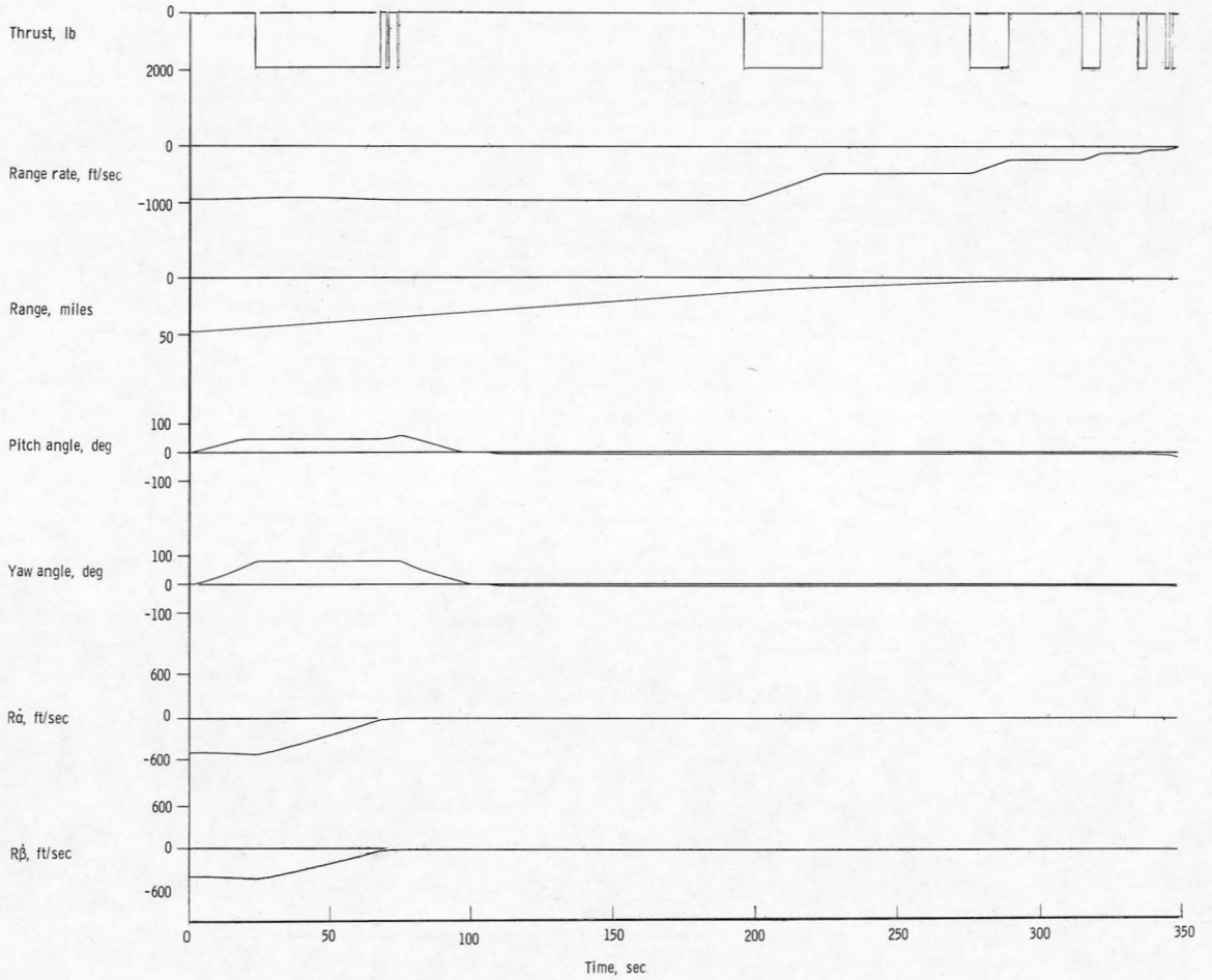
Figure 9.- Time history of the terminal phase of rendezvous for on-off thrust control.
