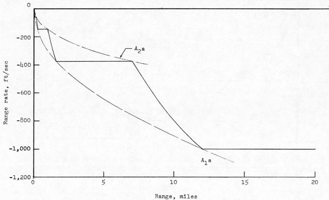
(c) A_1a = 8 \text{ ft/sec}^2 ; A_2a = 2 \text{ ft/sec}^2 .
