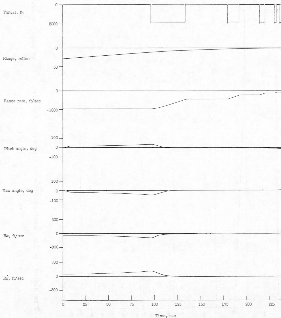
Figure 11.- Time history of the control of residual normal velocity components during braking for system employing on-off thrust control.
