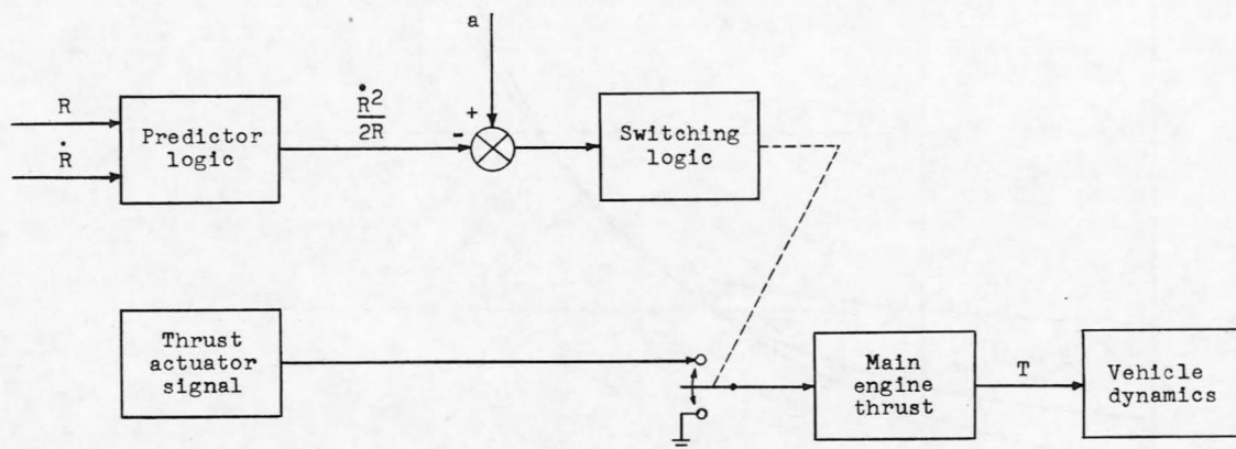
(b) On-off thrust control.
