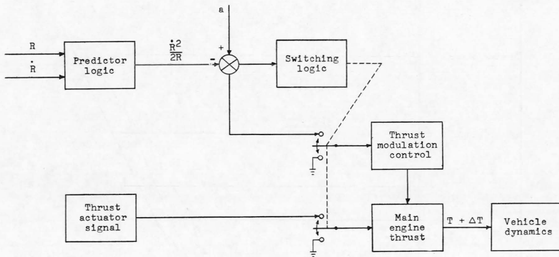
(a) Modulated thrust control.
