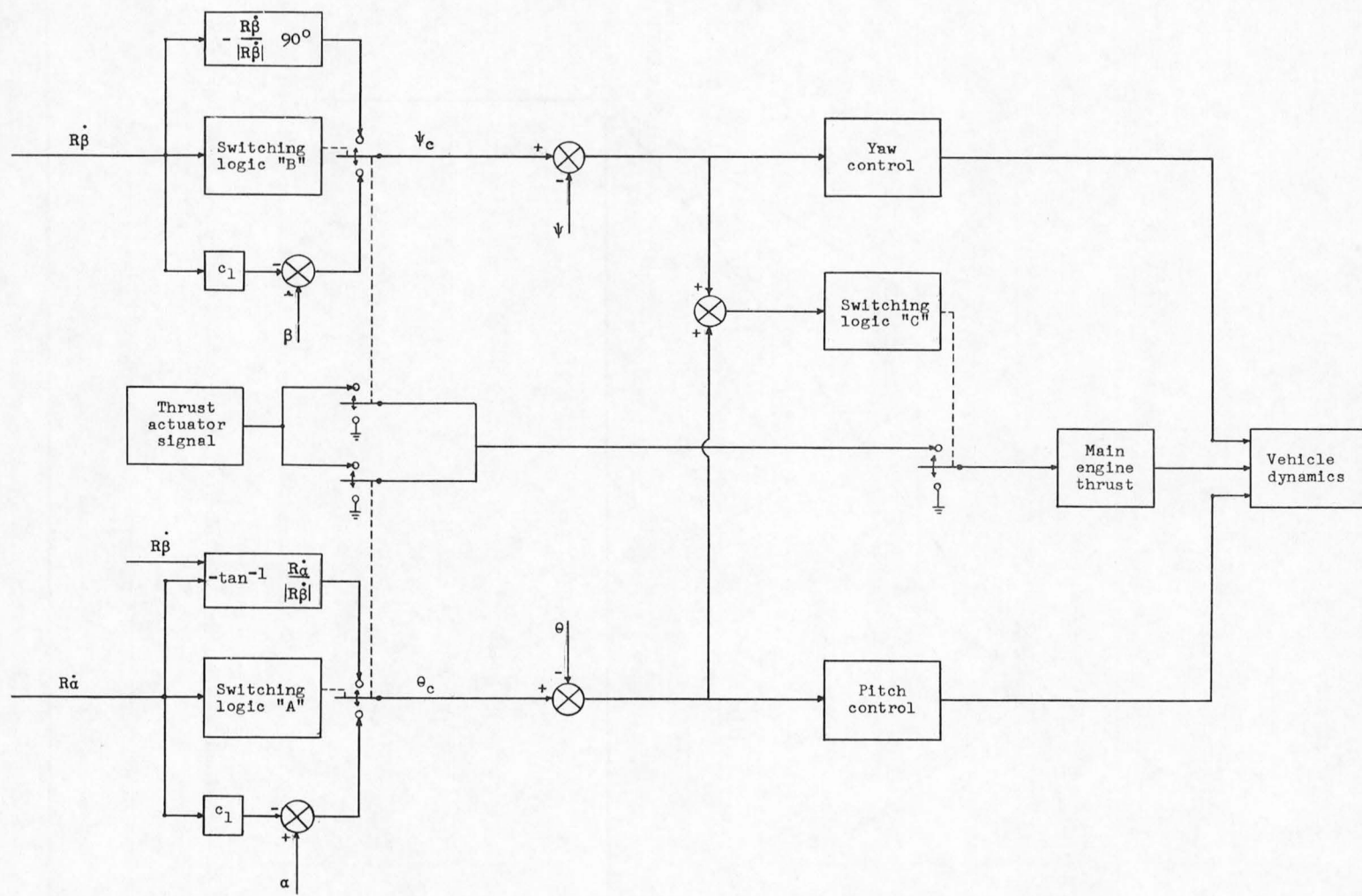
Figure 3.- Normal-velocity control.
