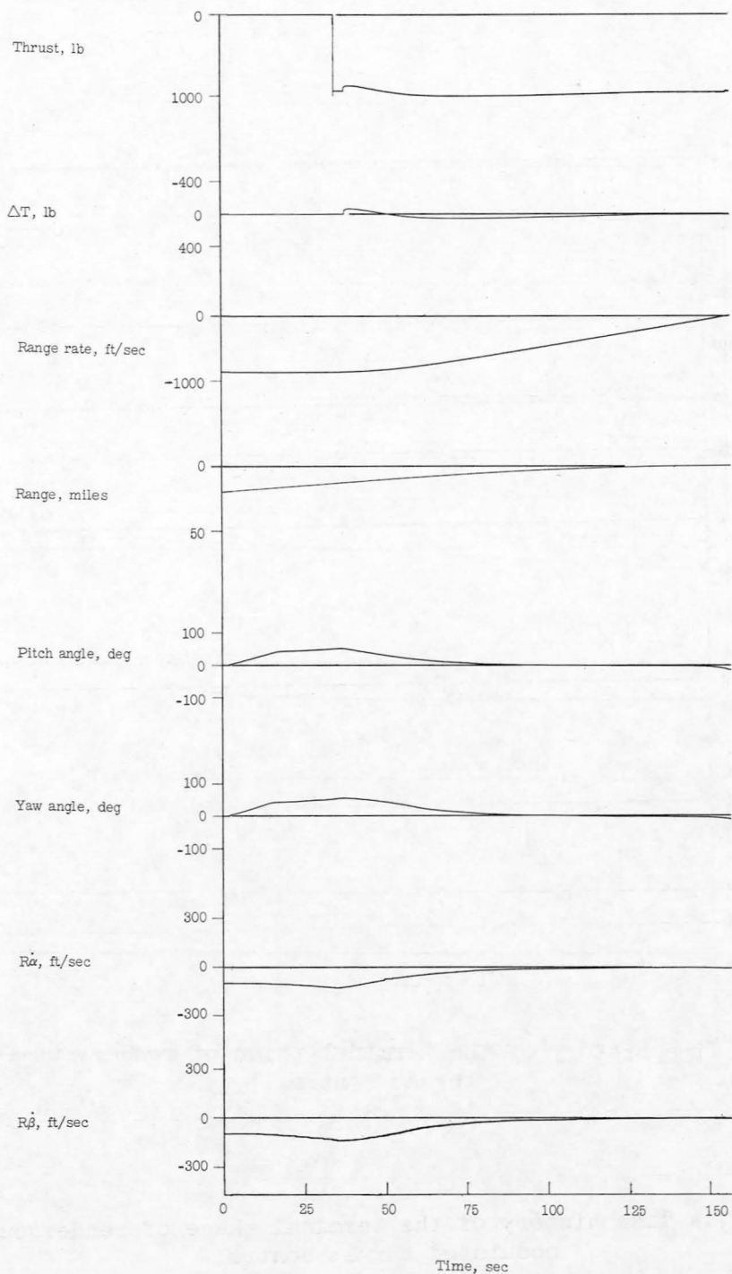
Figure 8.- Time history of the control of residual normal velocity components during braking for system employing modulated thrust control.
