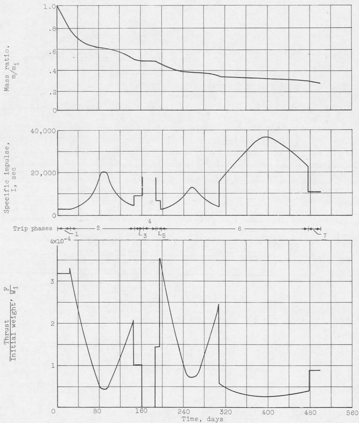
Figure 11. - Time history of mass, thrust, and specific impulse for 500-day and 800-day Mars round trips ( \alpha = 10 lb/kw, \beta = 0.20 ).
