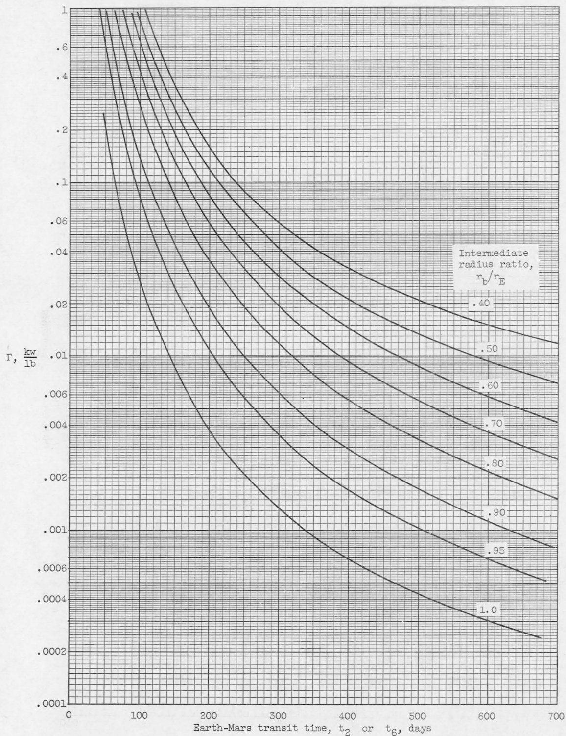
Figure 8. - Values of \Gamma for Earth-Mars transfers.
