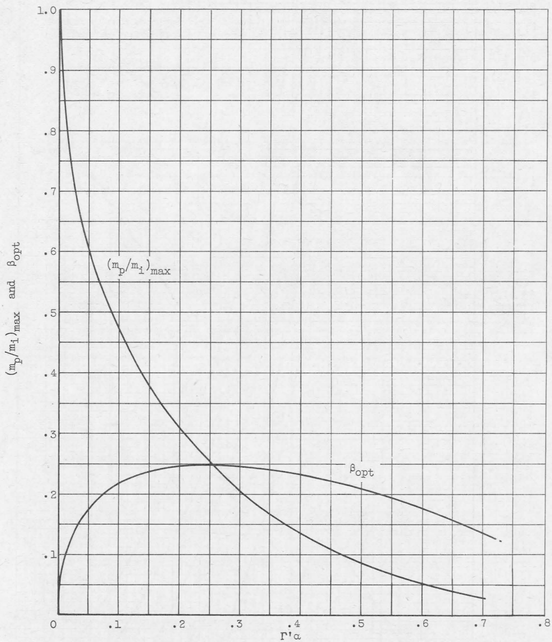
Figure 2. - Optimum powerplant mass ratio and maximum payload ratio as functions of \Gamma'\alpha for m_l/m_i = 1.0 .
