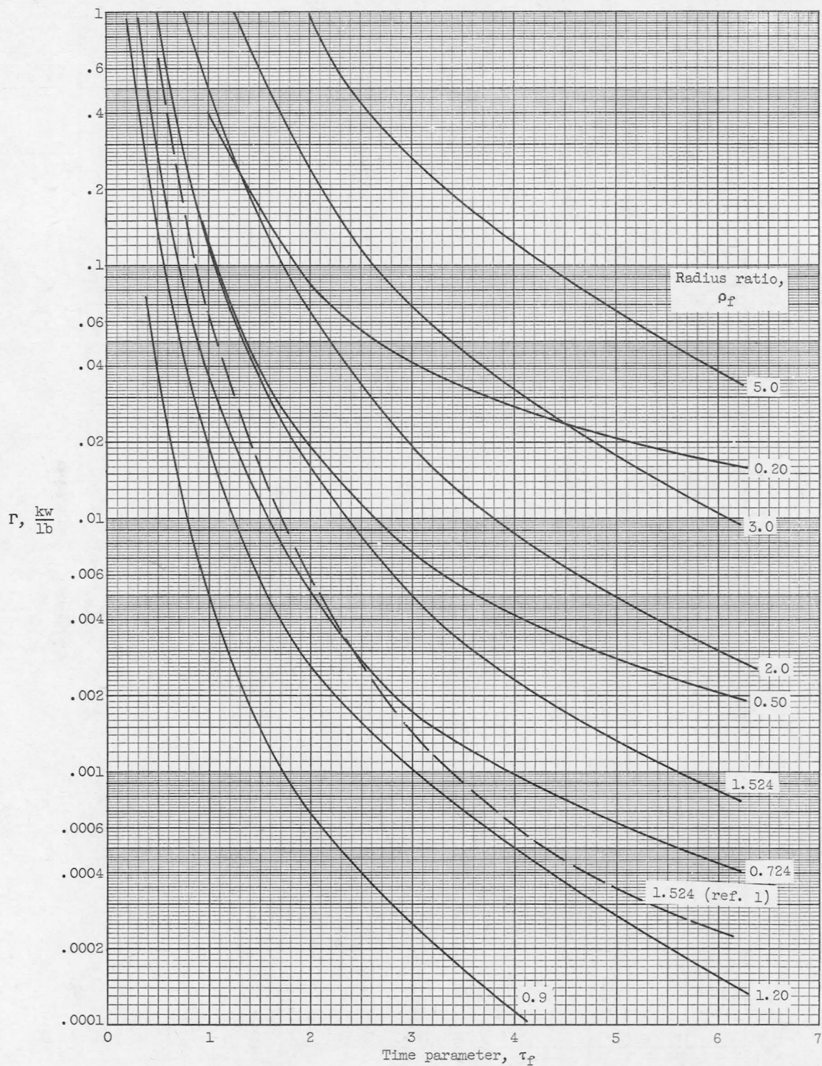
Figure 4. - Values of \Gamma for \theta' = \rho^{-3/2} trajectories.
