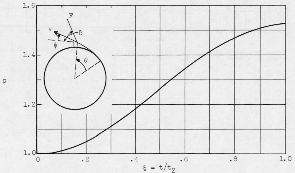
Figure 12. - Time history of several trajectory variables for Earth-Mars transfer along \theta' = \rho^{-3/2} trajectories.
