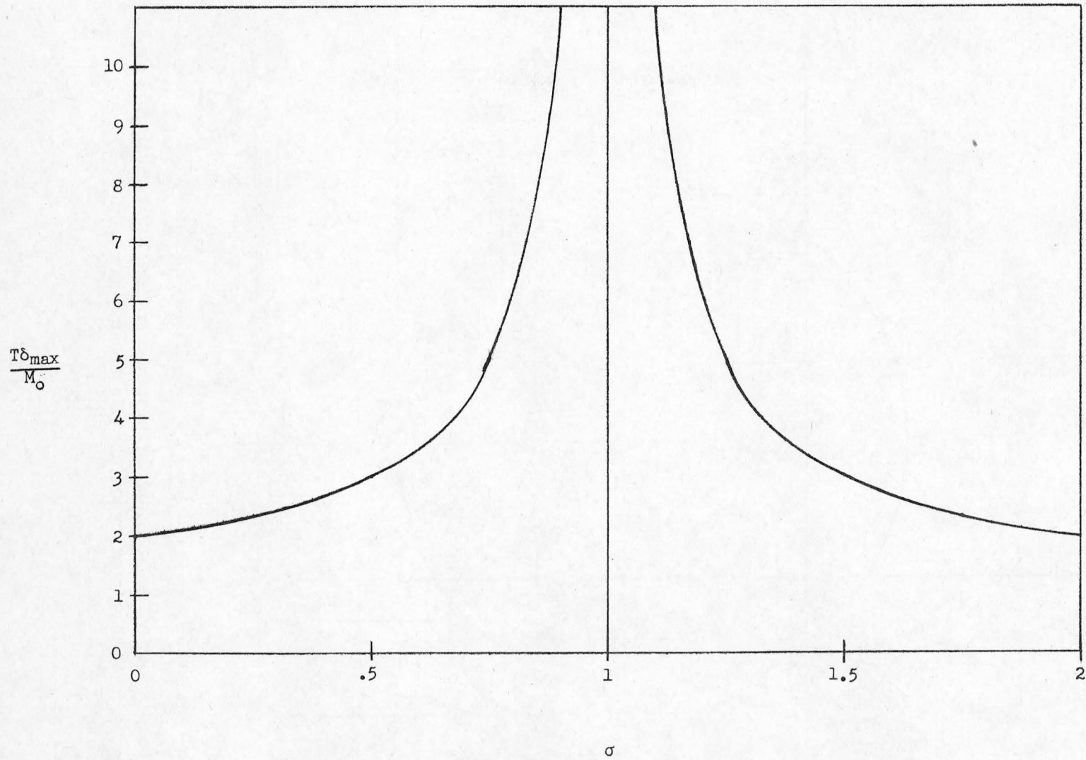
Figure 5.- Chart for determining the required spin kinetic energy or the maximum angular deflection in the equilibrium state for a spin-stabilized space vehicle.
