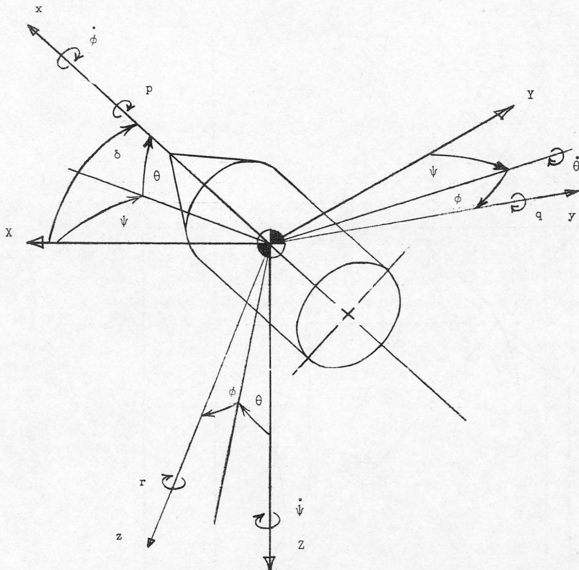
Figure 1.- Orientation of x, y , and z body axes relative to X, Y , and Z inertial axes. The relationship is described by the Euler angles \psi , \theta , and \phi . Positive sense of angular rates about body axes is shown as p, q , and r .
