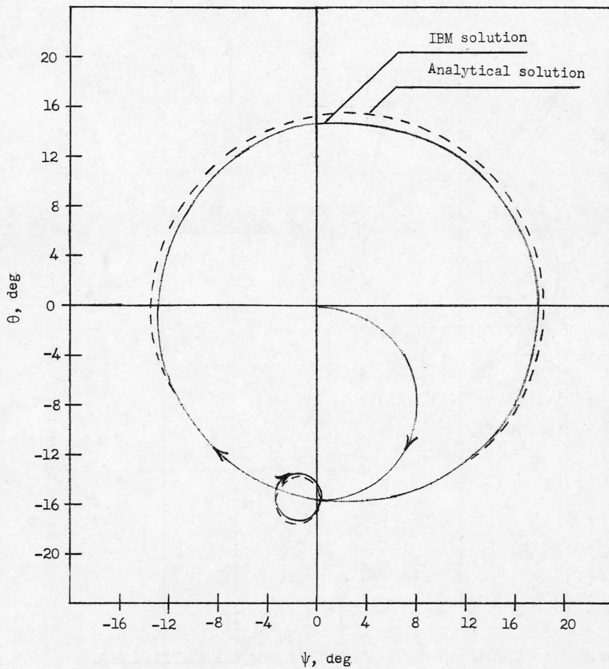
Figure 3.- Comparison of analytical results with IBM solutions of general equations of motion for two cases.
