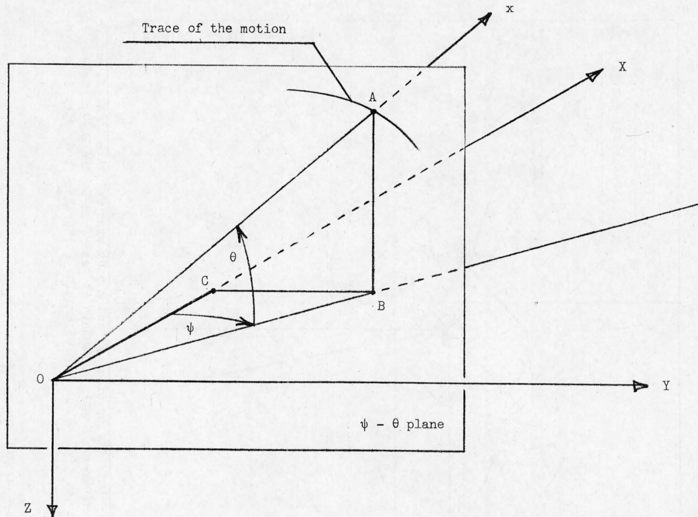
Figure 2.- Motion trace in \psi - \theta plane.
