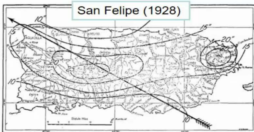
FIG. 1.—Rainfall distribution in Puerto Rico hurricane, September 13, 1928
