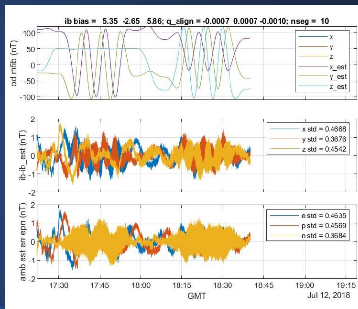
GOES-17 IB fields (top), background fit residual in IB frame (middle), and background fit residual in EPN/error estimate (bottom) from July 12, 2018 calibration maneuver
