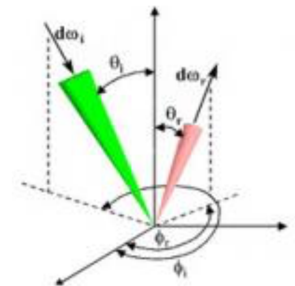
Bidirectional reflectance distribution function (BRDF)
