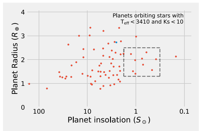
Figure 11. Planets make good targets for transmission spectroscopy if they orbit bright, small stars. This plot shows planets that orbit stars with spectral type M3V or later and that are brighter than K_s = 10 . The box is an approximate region showing planets that may have somewhat extended atmospheres (i.e., super-Earths) and are in the circumstellar habitable zone. There are 10 planets within this region, making up the prime JWST target sample from TESS .
