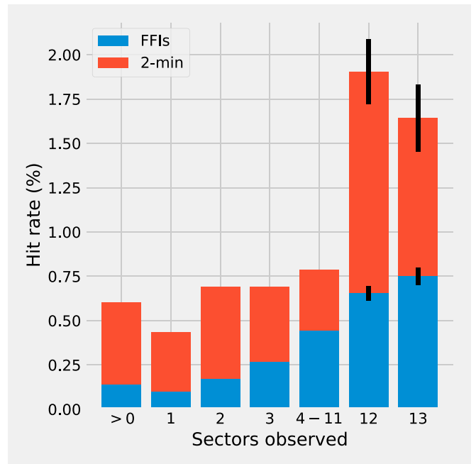
Figure 7. Ratio of stars observed to planets detected as a function of the number of sectors a star is observed for. The longer a star was observed, the higher probability a planet would be detected. Targets observed at 2-minute cadence are shown in red, while blue are FFI targets. For 2-minute cadence stars the average hit rate was 0.60%, while including all stars on the CTL drops this to 0.14%. While observing for a longer baseline increased the number of planets, the increase is not linear. For 2-minute cadence targets, an increase of 12 \times in observing baseline increased the hit rate by a factor of just 4.4. There are comparatively few planets in the 12 and 13 sector bins, so we show Poisson uncertainties on these bars demonstrating that there is not a measurable difference between observing for 12 or 13 sectors. Red and blue bars are not stacked; both start at zero.
