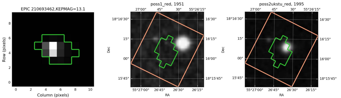
Figure 6. Archival imaging data for K2-288. The left panel is the data from K2 in 2015 with the k2_{\text{phot}} optimal photometric aperture overlaid in green. The center panel is a POSS I R_{\text{POSS}} -band image from 1951. The right panel is a POSS II R_{\text{POSS}} -band image from 1995. The optimal aperture is translated into the POSS image coordinates for comparison. K2-288 has moved substantially over the nearly 65 years covered by the images. The lack of a bright star at the current position of K2-288 in the past images indicates that there are no background sources at its current position that remain unresolved in our AO imaging observations and that the imaged companion is co-moving with the primary. We also note the faint, slow moving background source just to the NE of the optimal aperture in the POSS images. Analysis of the transit depth using different size apertures indicates that this star is not the source of the transit signal.
