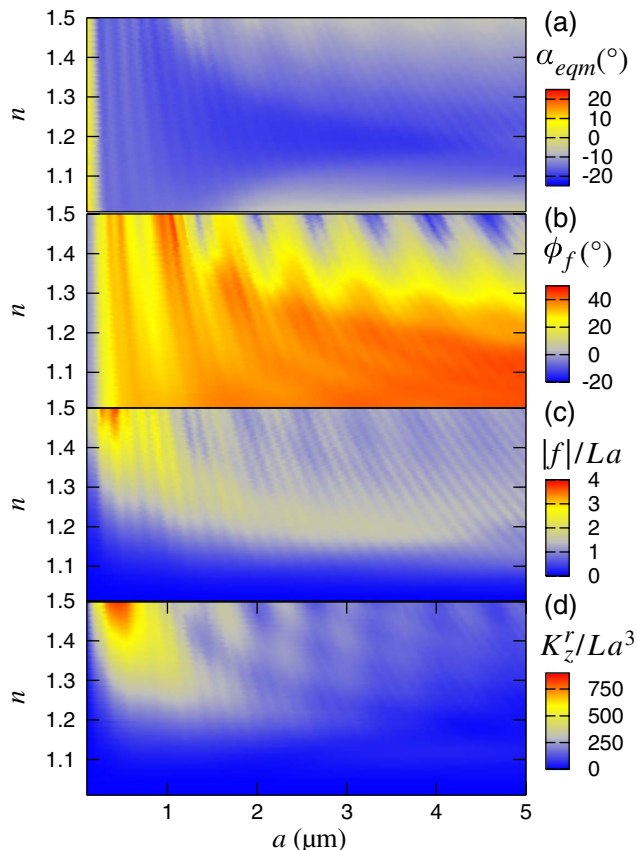
Fig. 4. (Color online) (a) Angle of attack at equilibrium, \alpha_{eqm} , (b) lift angle, \phi_f , (c) scaled force modulus, |f|/La ( \text{pN}/\mu\text{m}^2 ), and (d) scaled torsional stiffness, K_z^r/La^3 ( \text{pN}/\text{deg} \cdot \mu\text{m}^3 ), as functions of n and a .
