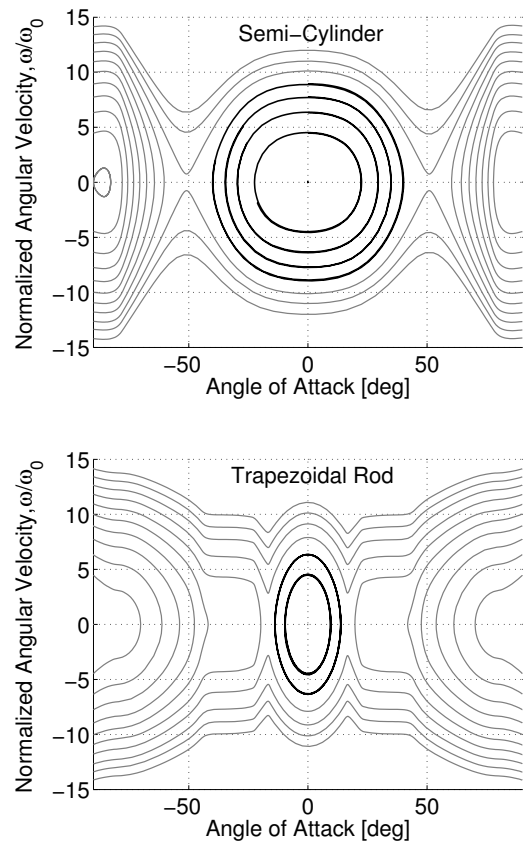
Fig. 3: Phase diagram at n = 1.5 for (a) semi-cylinder and (b) trapezoidal rod. Contours separated by 10[J\omega_0^2] .
