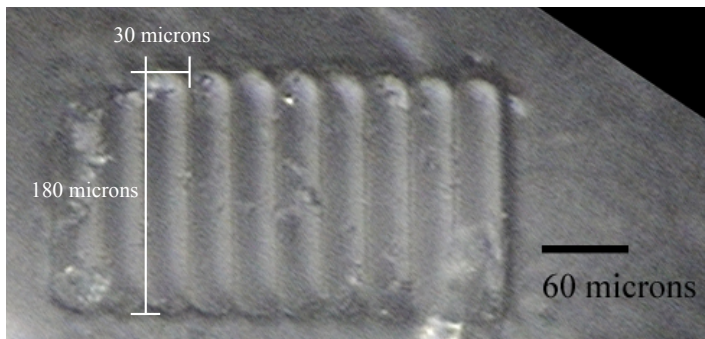
Figure D – 50x microscopic image of the smallest fabricated flying carpet made out of silicon elastomer. Defects in the semi-cylindrical features are due to tearing of the elastomer while releasing it from the mold.
