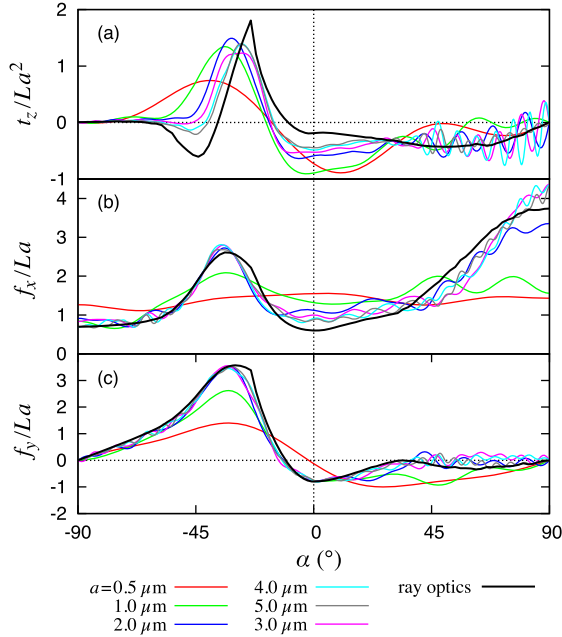
Fig. 2. (Color online) Forces and torques experienced by lightfoils with n = 1.3 , L = 1 \mu\text{m} , and various radii, a . (a) Scaled axial torque, t_z/La^2 (pN/ \mu\text{m}^2 ), (b) scattering force, f_x/La , and (c) lift force, f_y/La (pN/ \mu\text{m}^2 ).
