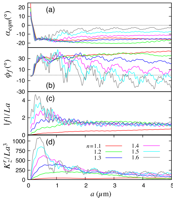
Fig. 3. (Color online) Stable equilibrium conditions for lightfoils of length 1 \mu\text{m} , with six distinct refractive indices, and 0.1 < a < 5 \mu\text{m} . (a) Angle of attack, \alpha_{\text{eqm}} , (b) lift angle \phi_f , (c) scaled force modulus, |f|/La (pN/ \mu\text{m}^2 ), and (d) scaled torsional stiffness, K_z^r/La^3 (pN/deg/ \mu\text{m}^3 ).
