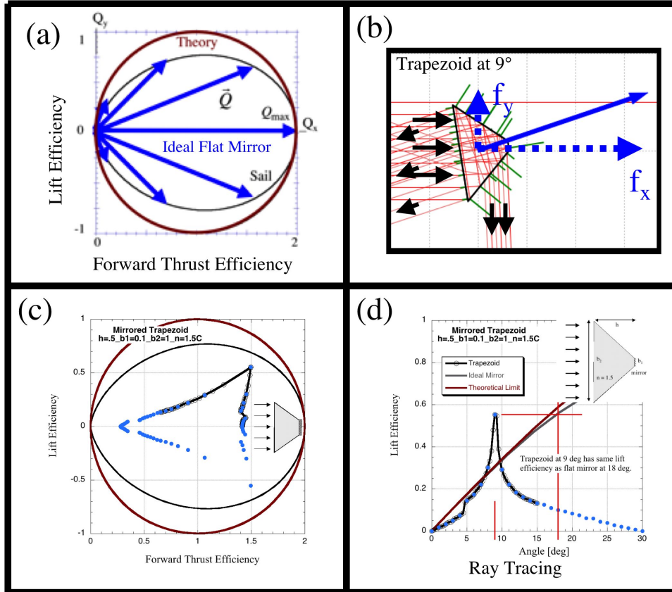
Figure 2. (a) Efficiency of radiation pressure force of a flat reflecting sail (blue arrows) does not achieve the theoretical limit (dark red circle) allowed by the conservation of momentum. (b) Ray tracing for a trapezoid, shown at an angle of attack of 9^\circ . (c) Same as (a) but with the parametric efficiency curve for a trapezoid. (d) Lift efficiency as a function of angle of attack, showing lift values greater than a flat reflector at 9^\circ .
