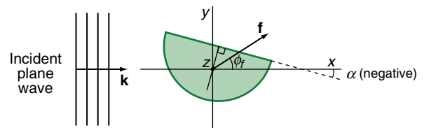
Fig. 1. (Color online) Schematic showing the axes and angles used in the text. The angle of attack, \alpha , and the angle at which the excess force acts, \phi_f , are measured counterclockwise from the positive x -axis.
