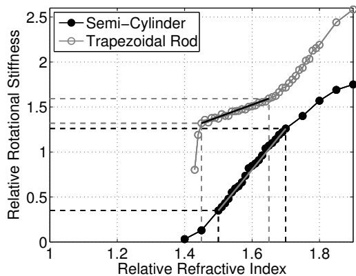
Fig. 4: Relative rotational stiffness against refractive index. Trapezoid curve is straight between 1.45 and 1.65, and semi-cylinder curve is straight between 1.5 and 1.7.
