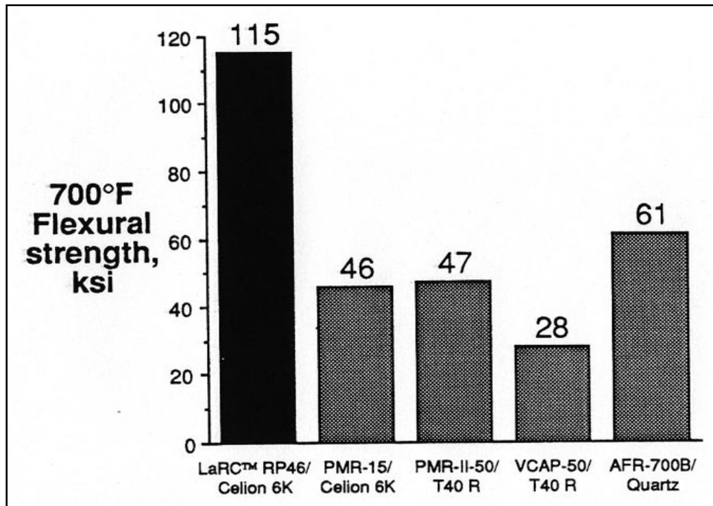
Figure 11.5-11: Flexure Strength at 700°F (371°C) for 5 PMR-Type Composites
