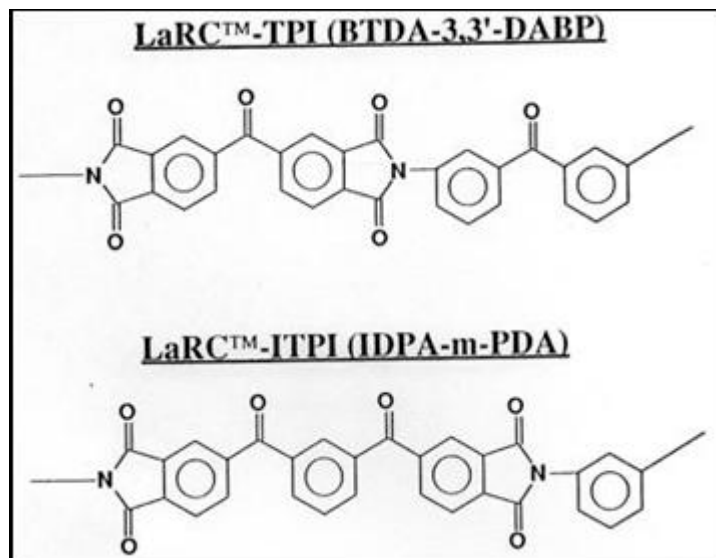
Figure 11.5-3: Isomeric Character of LARC™ TPI and LARC™ ITPI
