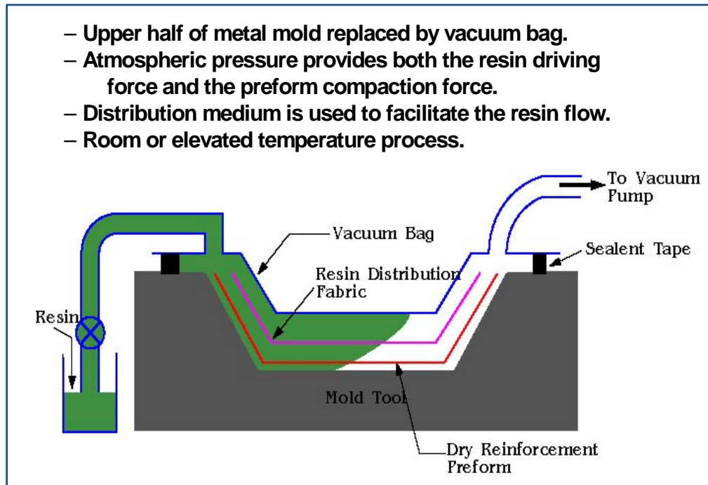
Figure 12.13-1: Equipment Set-up for VARTM. Courtesy of Dr. B. J. Jensen
