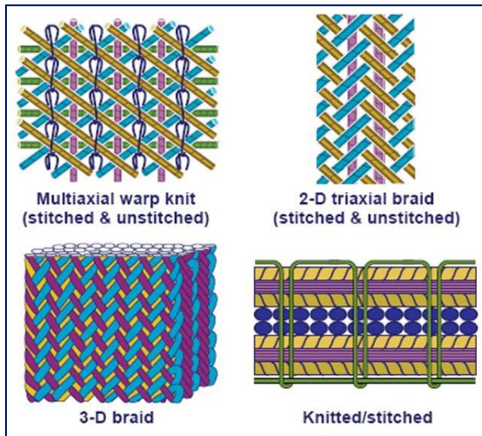
Figure 4.4-1: Textile Material Forms
