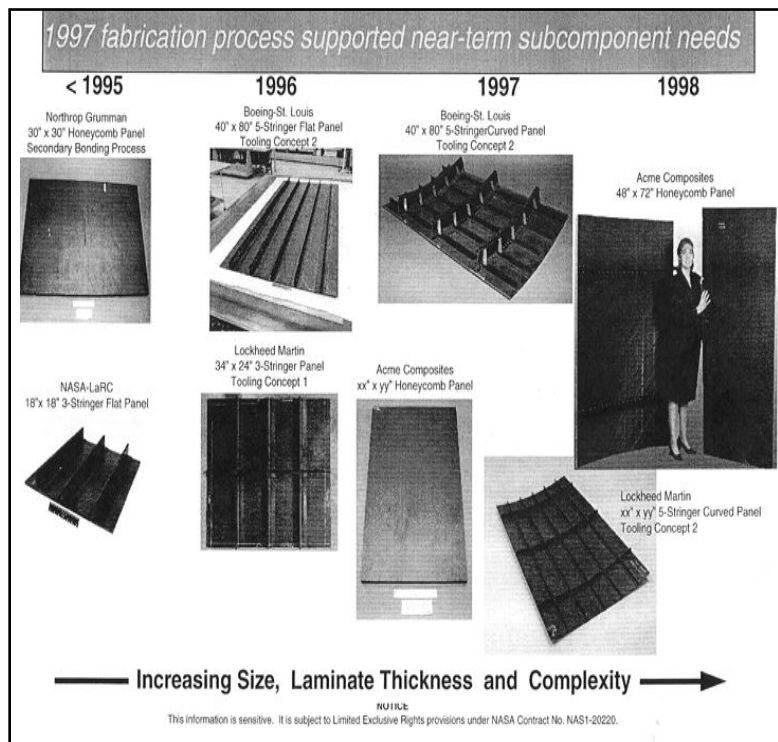
Figure 11.6-6: IM-7/LARC™-PETI-5 Composite Panels Autoclave Fabricated from Hand Layup Wet Prepreg
