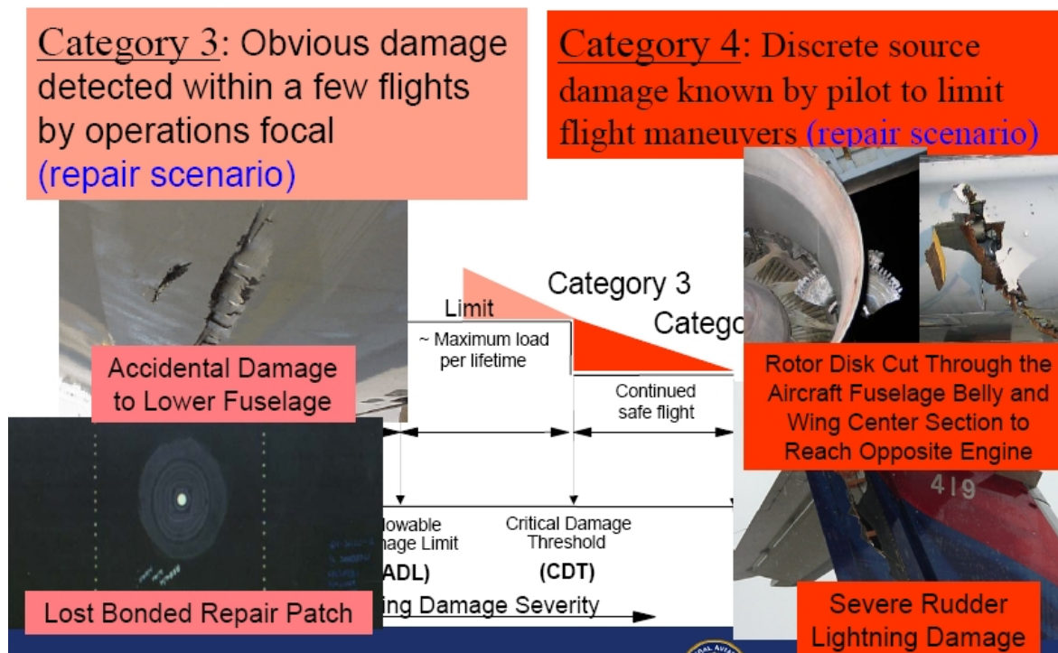
Figure 15.1-3: FAA Categories of Damage for Composite Aircraft Structure and Selected Examples of Damage on Actual Aircraft
