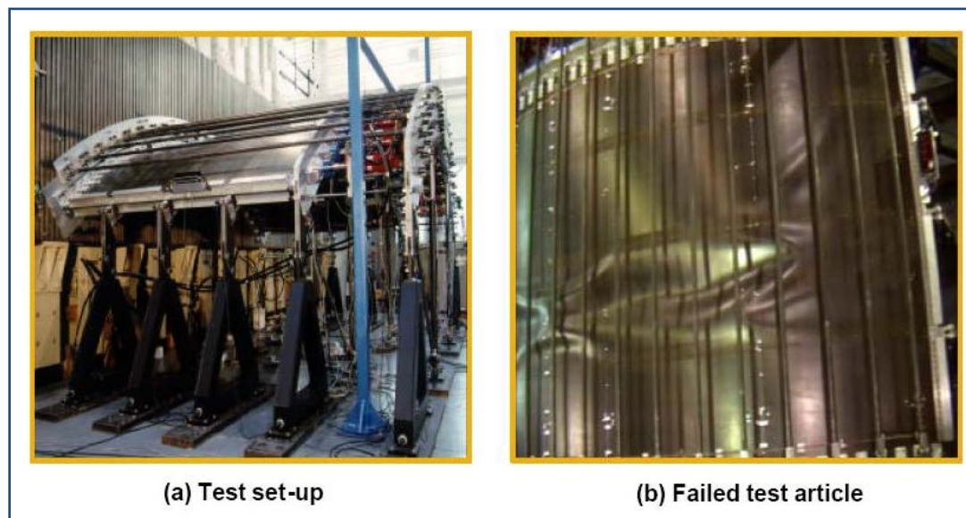
Figure 9.3-3: LaRC Structural Test of Segment of an RLV Intertank
