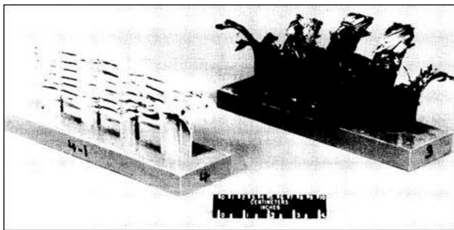
Figure 8.2-4: Crushed Kevlar/934 and T300/934 ((±45) 4 ) s Circular Tube Stiffened Beams
