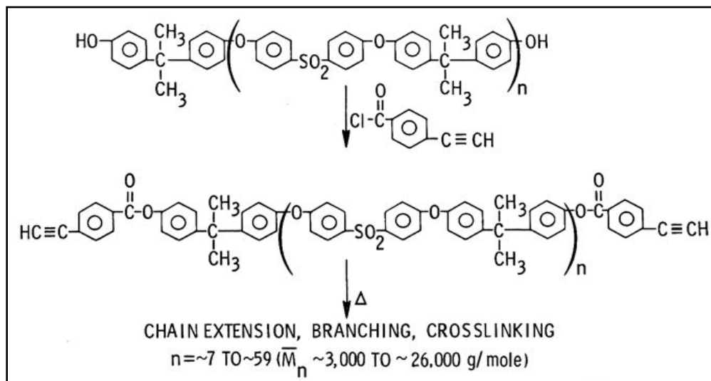
Figure 11.5-10: Formation of Ethynyl-terminated Polysulfones
