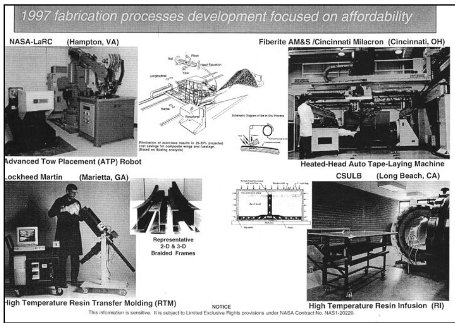
Figure 11.6-5: Advanced Fabrication Techniques Developed During the HSR Program
