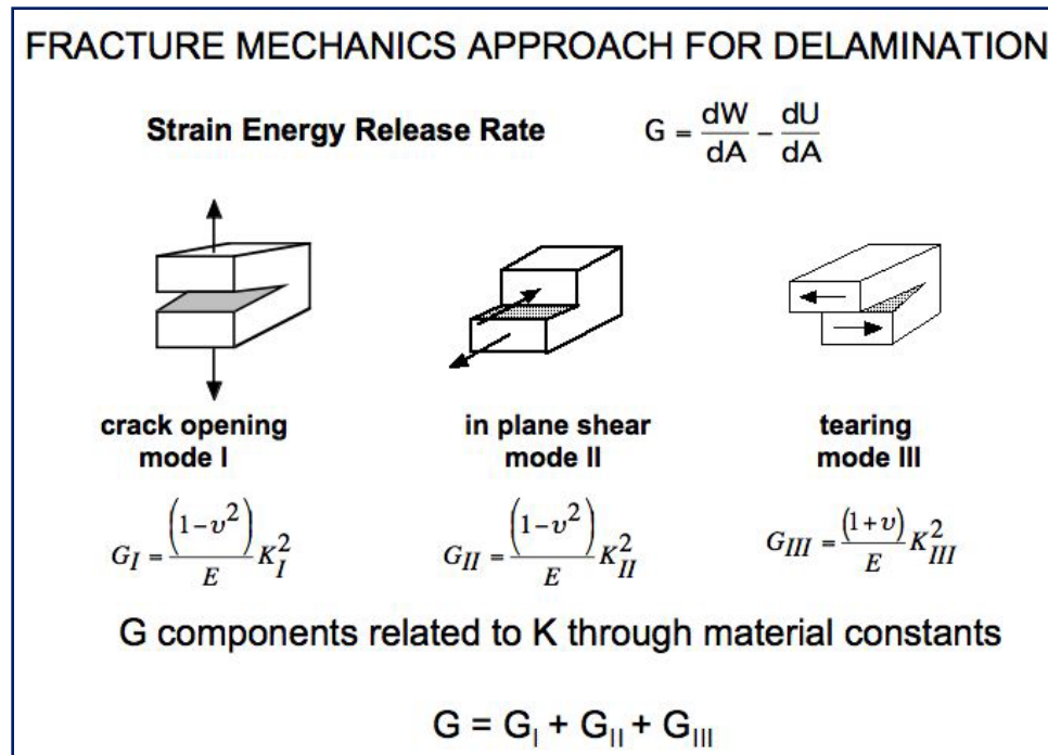
Figure 15.2-6: Fracture Mechanics Approach for Delamination (Courtesy of T. K. O'Brien and J. R. Reeder, LaRC, 2007)
