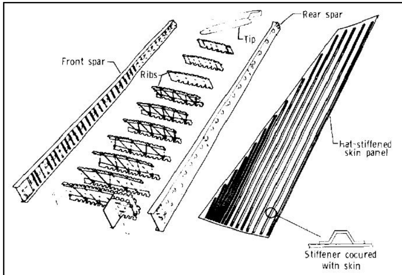
Figure 4.2-8: Graphite-Epoxy Vertical Fin on L-1011
