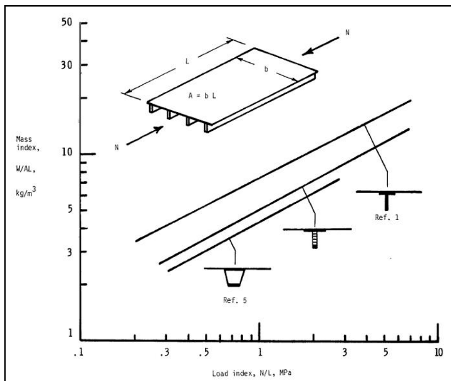
Figure 16.3-3: Compression-load Structural Efficiency Comparison For Graphite/epoxy Blade, Sandwich-Blade and Hat-Stiffened Panels
