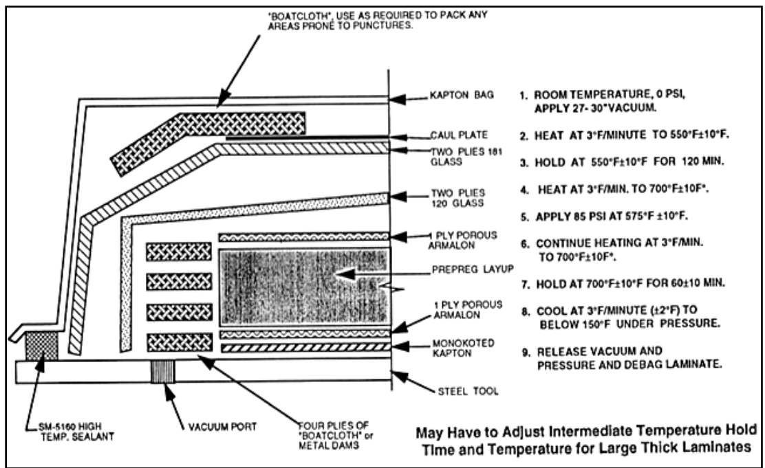
Figure 11.6-4b: Recommended Bagging for Processing LARC™-PETI-5 IM-7 Composites
