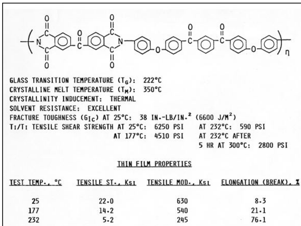
Figure 11.5-5: Chemical Structure and Properties of LARC-CPI Polymer
