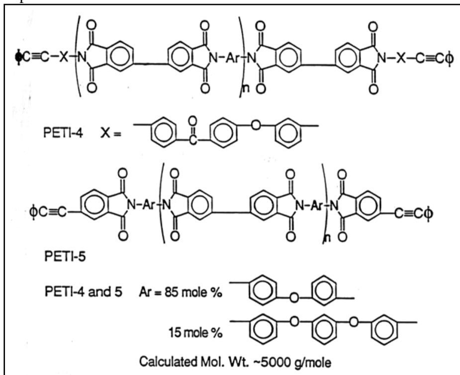
Figure 11.6-1: Chemical Structures of LARC™-PETI-4 and LARC™-PETI-5
