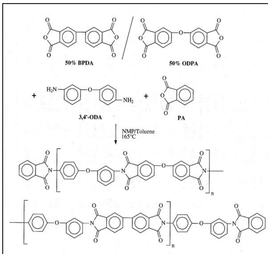
Figure 11.5-6: Synthetic Scheme For LARC TM -SI
