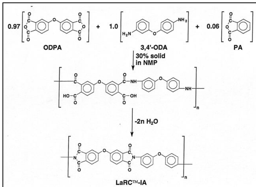
Figure 11.5-4: Synthesis of LARC™ IA With 3% Stoichiometric Offset
