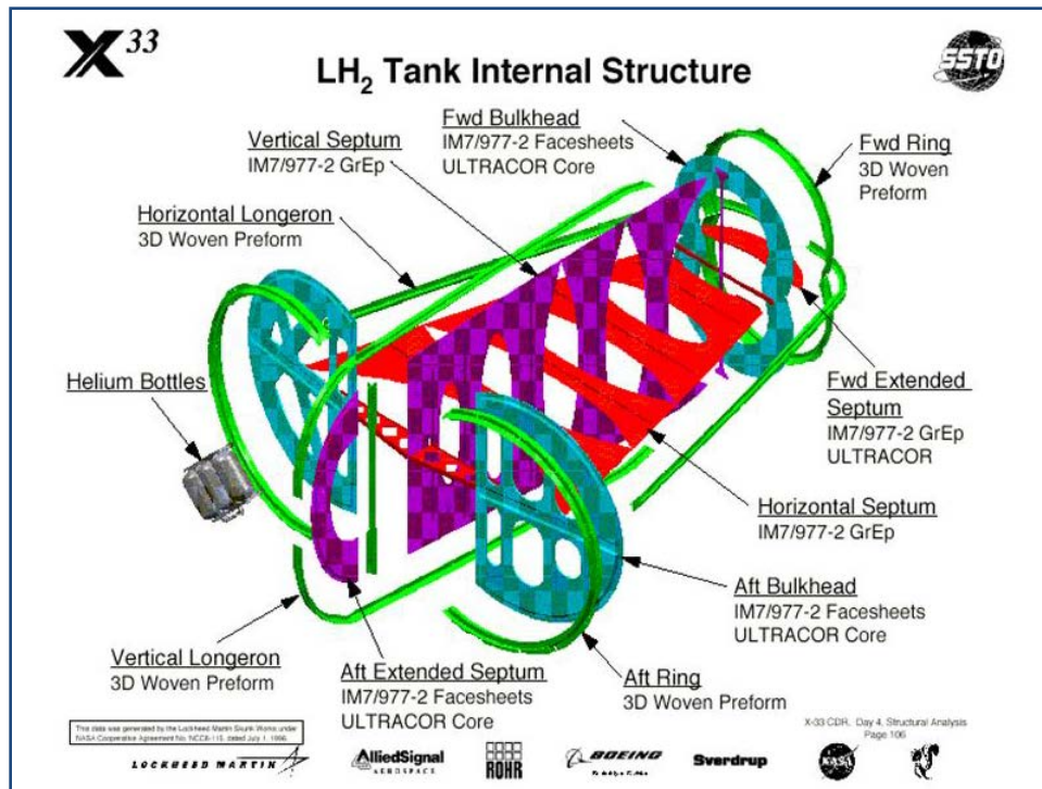
Figure 9.3-7: Composite LH 2 Internal Tank Structure showing the 4 Longérons (green) and the 2 Septums (purple and red)
