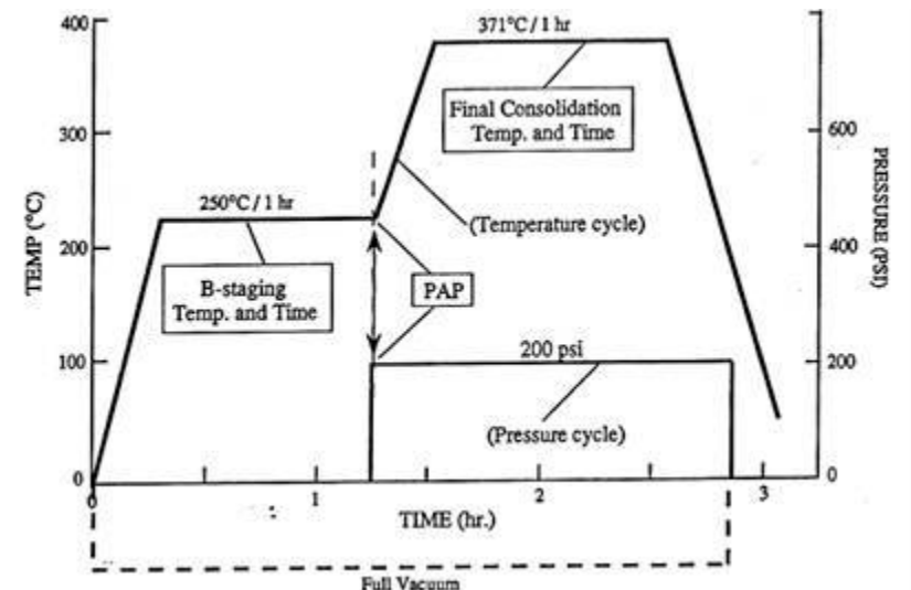
Figure 11.6-4a: Recommended Cure Cycle for Processing LARC™-PETI-5 IM-7 Composites
