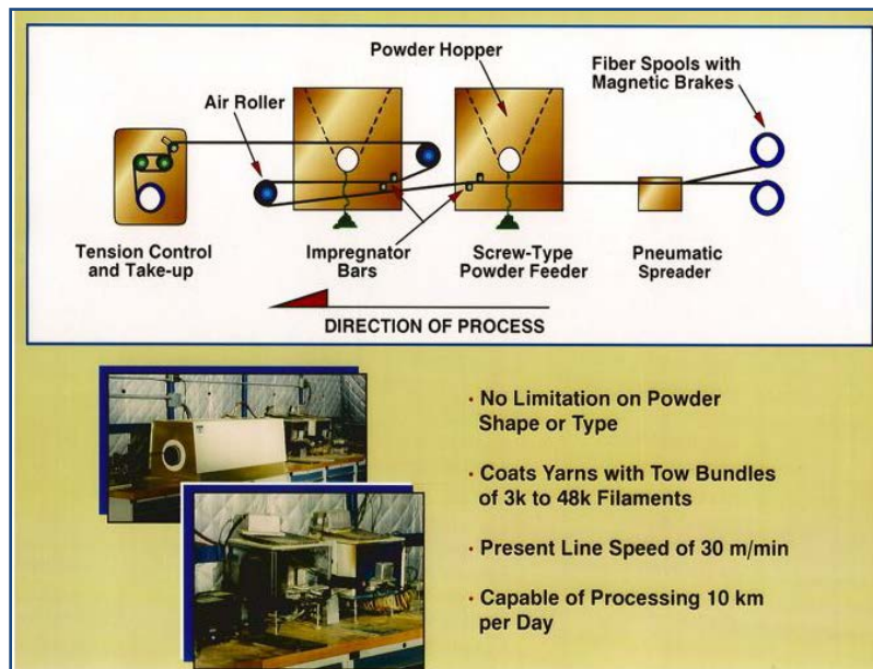
Figure 12.6-3: Schematic of Hoppers in the Dry Powdercoating Line
