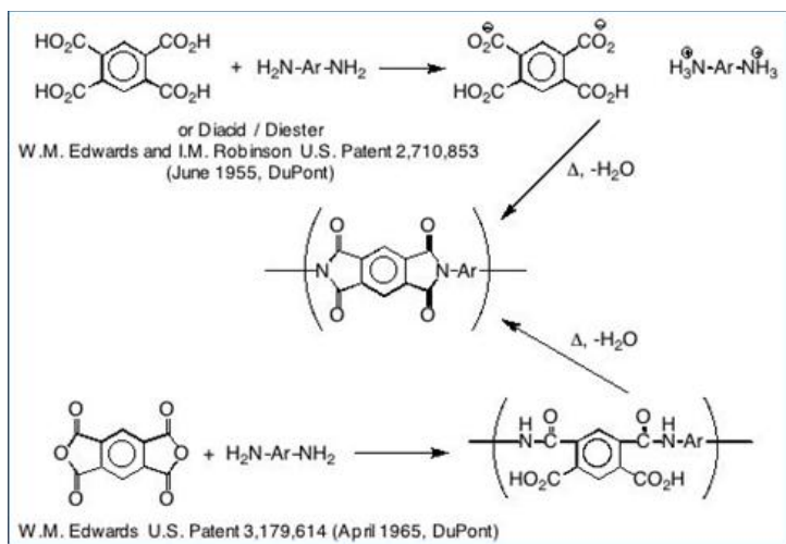
Figure 11.3-2: DuPont's Aromatic Polyimide Chemistry Showing the Critical Prepolymer Poly(amide acid) in the Lower Right.
