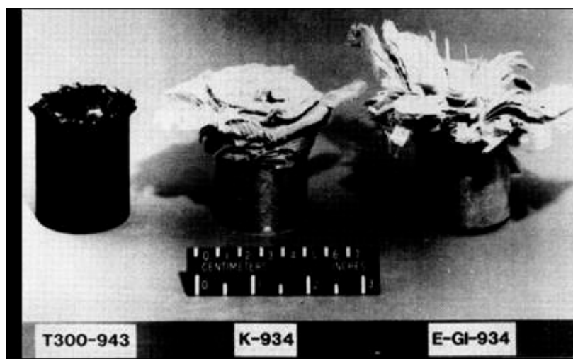
Figure 8.2-3 Crushing Modes for (0/±45/90)s Composite Tubes
