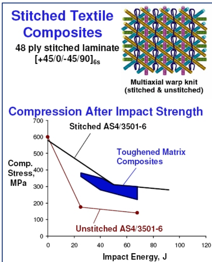
Figure 4.4-2: Stitching Improves Damage Tolerance
