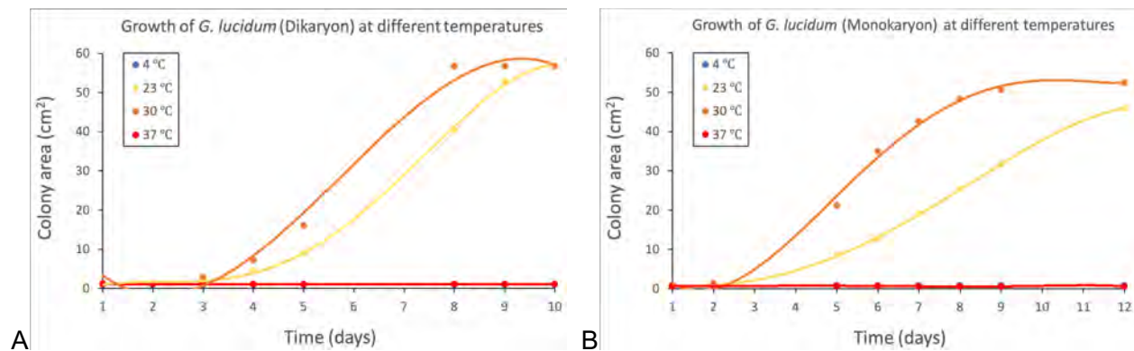
Figure 6. Growth dynamic of Ganoderma lucidum Dikaryon (A) and Monokaryon (B) under different temperatures, as measured by colony area (cm 2 ).
