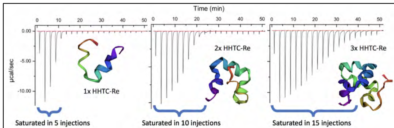
Figure 12. ITC data for the three HHTC-Re peptides. The binding affinity ( K_a ) was assessed to determine the strength of the interaction, and the results follow: 1x-HHTC-Re K_a = (1.55 \pm 0.21) \times 10^6 \text{ M}^{-1} ; 2x-HHTC-Re K_a = (3.73 \pm 0.53) \times 10^5 \text{ M}^{-1} ; 3x-HHTC-Re K_a = (1.50 \pm 0.05) \times 10^5 \text{ M}^{-1} . Figure design credits to Jesica Urbina.
