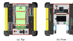
Fig. 2. Snapshot of the Astrobee payload bay.
