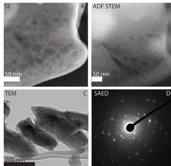
Figure 1: TEM data of grains after irradiation. A) SE image of the 3.5 \times 10^{16} ions/cm 2 irradiated grain showing surface depressions corresponding to vesicles in the B) ADF image. C) TEM image of vesicles in the sample irradiated to 5 \times 10^{16} ions/cm 2 and D) Selected-area electron diffraction pattern containing discrete reflections and rings, indicating the start of amorphization.
