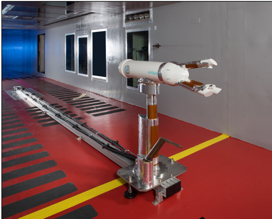
Figure 1.—Artium Technologies, Inc. PDI-FPDR and pitot-static probe mounted upstream in the IRT contraction.
