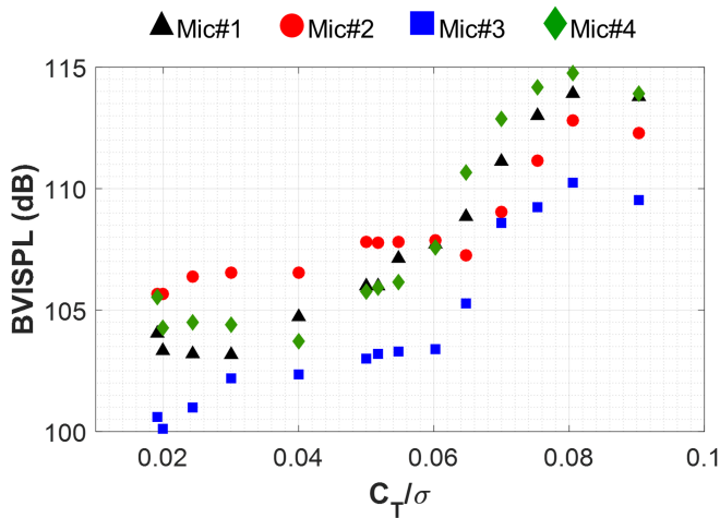
Fig. 15. TTR in the NFAC 40- by 80-Foot Wind Tunnel BVISPL versus C_T/\sigma for microphones 1 through 4 for a flight condition of \mu = 0.125 , M_{tip} = 0.684 , and \alpha_s = 0^\circ .
