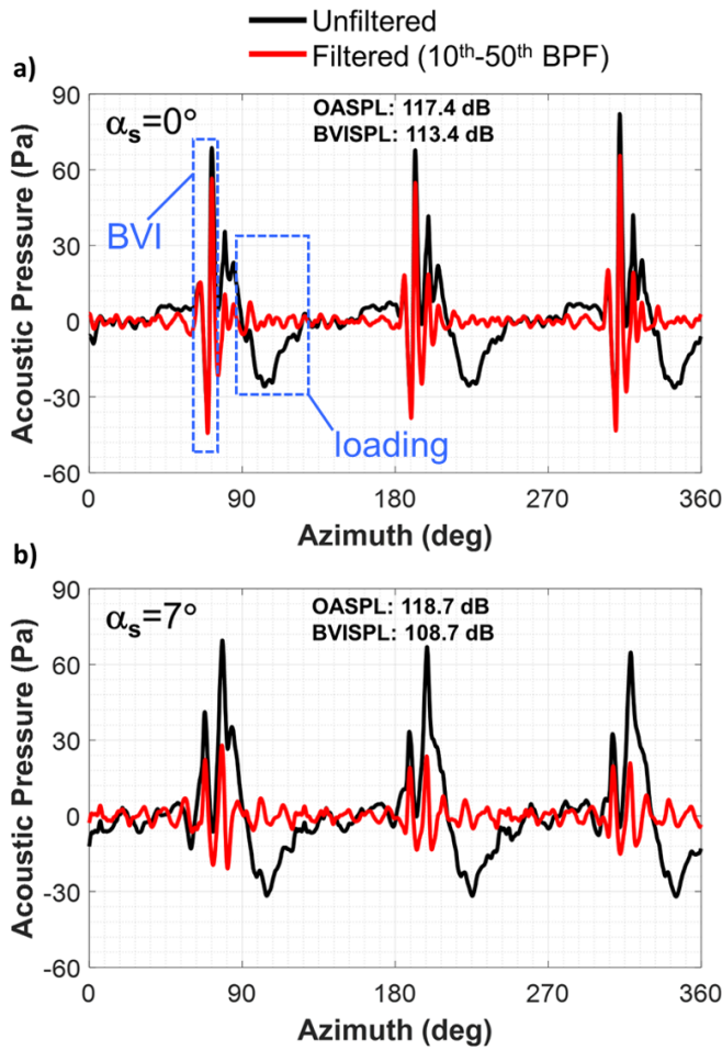
Fig. 14. TTR in the NFAC 40- by 80-Foot Wind Tunnel unfiltered and filtered acoustic time history for microphone 1 for a flight condition of C_T/\sigma = 0.075 , \mu = 0.125 , M_{tip} = 0.684 , at a) \alpha_s = 0^\circ and b) 7^\circ .
