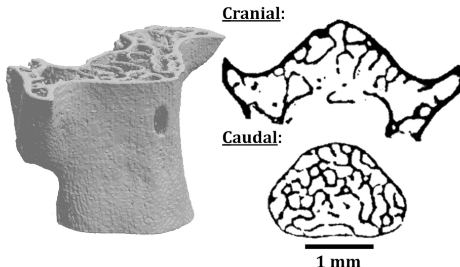
Fig. 2. Representative sample of a mouse vertebral body after all specimen preparation. Cranial and caudal cross-sections shown at 10- \mu m voxel resolution.
