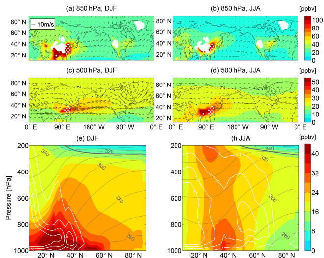
Figure 1. Ensemble mean of the horizontal distribution of CO 50 concentration (shades, units: ppbv) at levels of (a, b) 850 hPa and (c, d) 500 hPa, and ensemble mean of the zonal-mean CO 50 concentration cross sections (e, f) during (a, c, e) DJF and (b, d, f) JJA. In (a)–(d), horizontal winds ( u , v ) are overlaid as vectors, and regions of CO 50 sources are highlighted by white stipples within which CO 50 emission fluxes are larger than 0.4 \times 10^{-9} \text{ kg m}^{-2} \text{ s}^{-1} . In (e) and (f), isentropic surfaces are overlaid as dark gray isopleths (units: K), the tropopause is marked as the bold dark gray curve, and regional convective mass flux (CMF) over East Asia (110–140° E) is denoted by white contours (units: 10^{-3} \text{ kg m}^{-2} \text{ s}^{-1} ).
