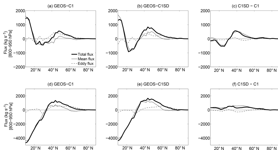
Figure 8. Tracer flux diagnostics showing the total flux ( \overline{v' \chi'_{CO50}} ) (heavy), zonal-mean flux ( \overline{v \chi_{CO50}} ) (light, solid), and eddy flux ( \overline{v' \chi'_{CO50}} ) (light, dashed) of CO50 (vertically integrated from 800 to 950 hPa; positive means northward; units: \text{kg s}^{-1} ) in (a) GEOS-C1, (b) GEOS-C1SD, and (c) the difference GEOS-C1SD–GEOS-C1 during summer. Panels (d), (e), and (f) are similar to (a), (b), and (c) but during winter. Results are based on the daily GEOS model output.
