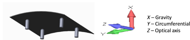
Fig. 5 Illustration of the four-point kinematic support of an x-ray mirror. The four supports are approximately located one quarter way inboard from each corner. See text for a discussion of the advantages of aligning and bonding a mirror segment using these four supports, which are also called spacers or posts.
