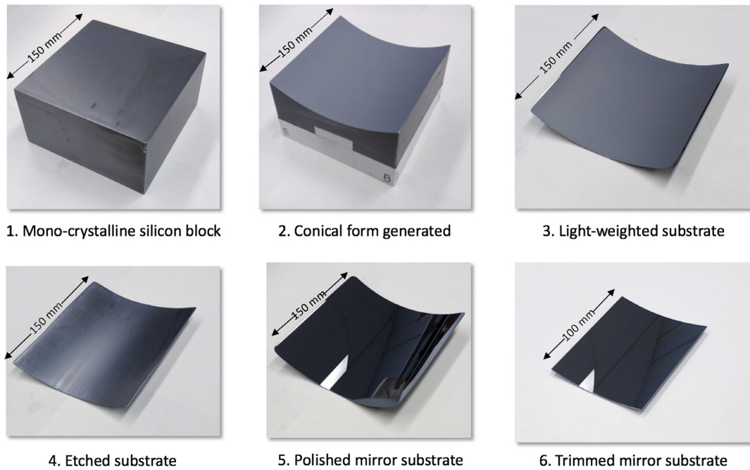
Fig. 2 Six major steps of fabricating a mirror substrate. This entire process, using no special equipment other than what is commonly available, takes about 15 h labor time and 1 week of calendar time. The process is highly amenable to automation and mass production methods, leading to high throughput and low cost.
