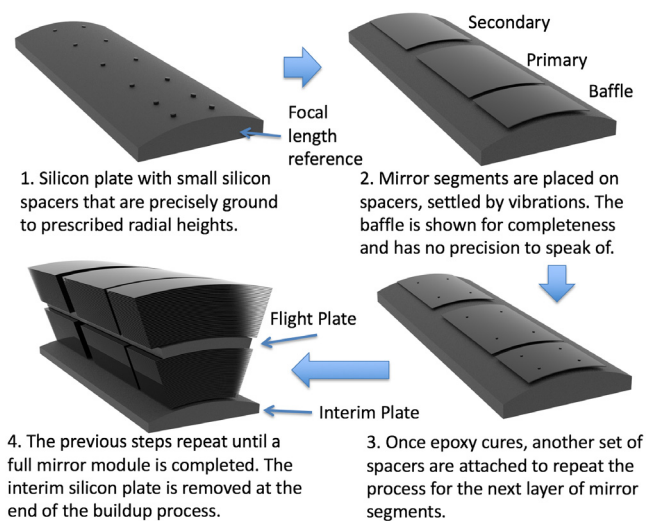
Fig. 8 Building-up of a mirror module. It is a repetition of fabrication, alignment, and bonding of one mirror segment after another. The interim plate is for the construction process only. It will be removed before the module is integrated into a metashell with the flight plate as its load-bearing structure and focal length reference.
