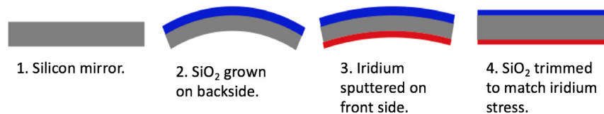
Fig. 4 Illustration of mirror coating process to enhance x-ray reflectance while preserving the figure quality of silicon substrate. The distortion caused by the stress of the iridium thin film is precisely balanced or compensated for by the stress of the silicon oxide on the other side of the mirror substrate.
