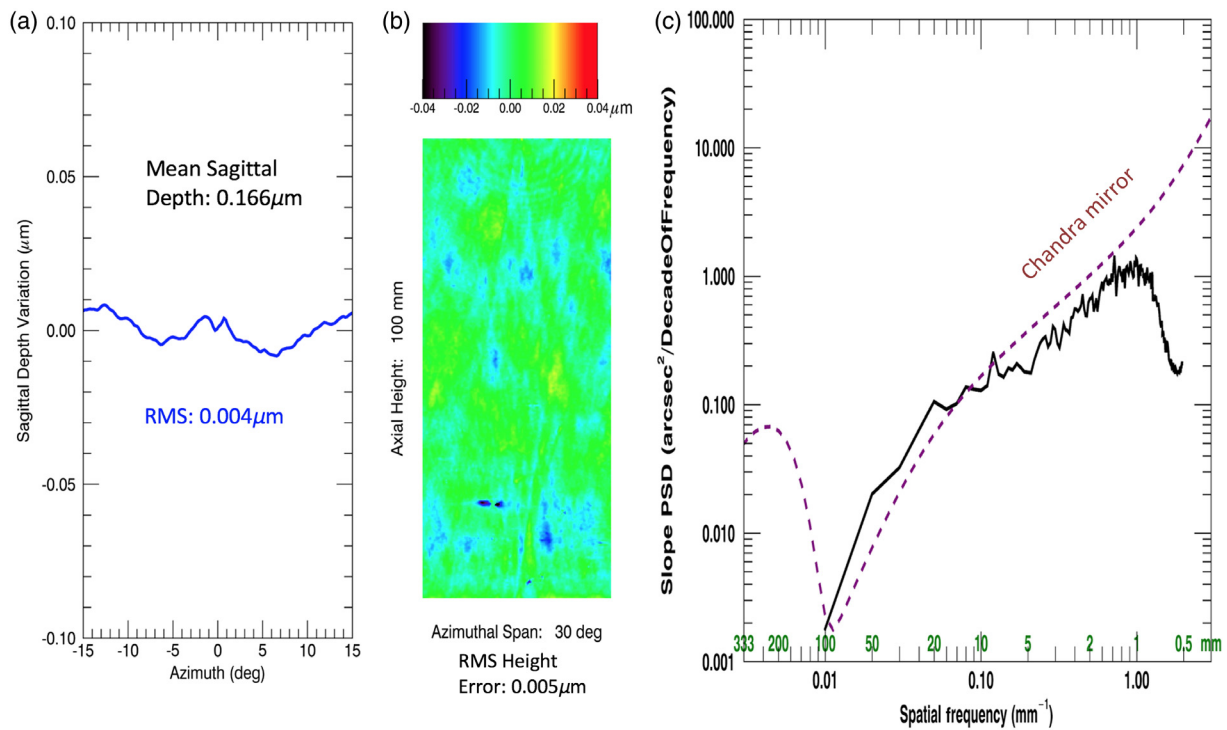
Fig. 3 Measured properties of a finished mirror substrate. (a) sagittal depth variation as a function of azimuth. This substrate's average sagittal depth of 166 nm differs from the design value of 174 nm by 8 nm. The RMS variation of the sagittal depth is 4 nm. (b) Surface error topography. After removal of the sagittal depth, this mirror has an RMS height error of only 5 nm. (c) Slope power spectral density (black solid curve) in comparison with Chandra's mirror (dashed curve). All of the errors combine to make this mirror substrate have an image quality of 0.5 arc sec HPD (two reflection equivalent).
