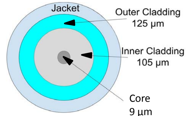
9/105 μm Double Clad Fiber
