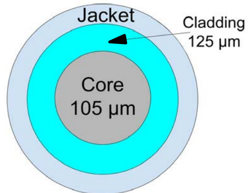
105 μm Multi Mode Fiber
