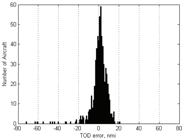
Figure 17. Error predicting TOD location for all flights. Negative values indicate flown distance is further from fix than predicted.
