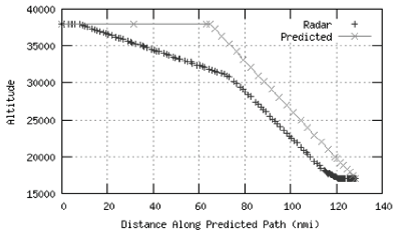
Figure 10. Vertical profile indicating two FPAs during descent.
