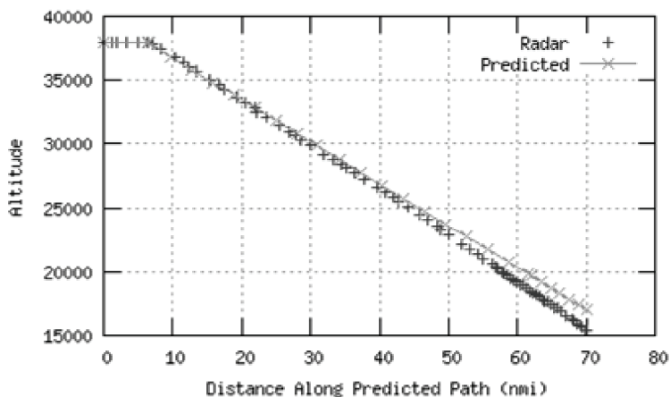
Figure 6. Vertical profile for SKW6901 on 10/31/2010 indicating the aircraft was not targeting the meter-fix altitude constraint.
