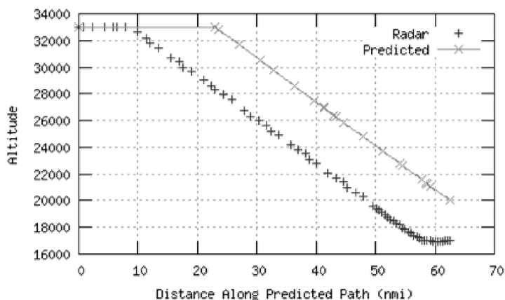
Figure 7. Vertical profile for SKW6896 on 11/10/2010 indicating the aircraft is targeting a different meter-fix altitude (17,000 ft) compared to prediction (FL200).
