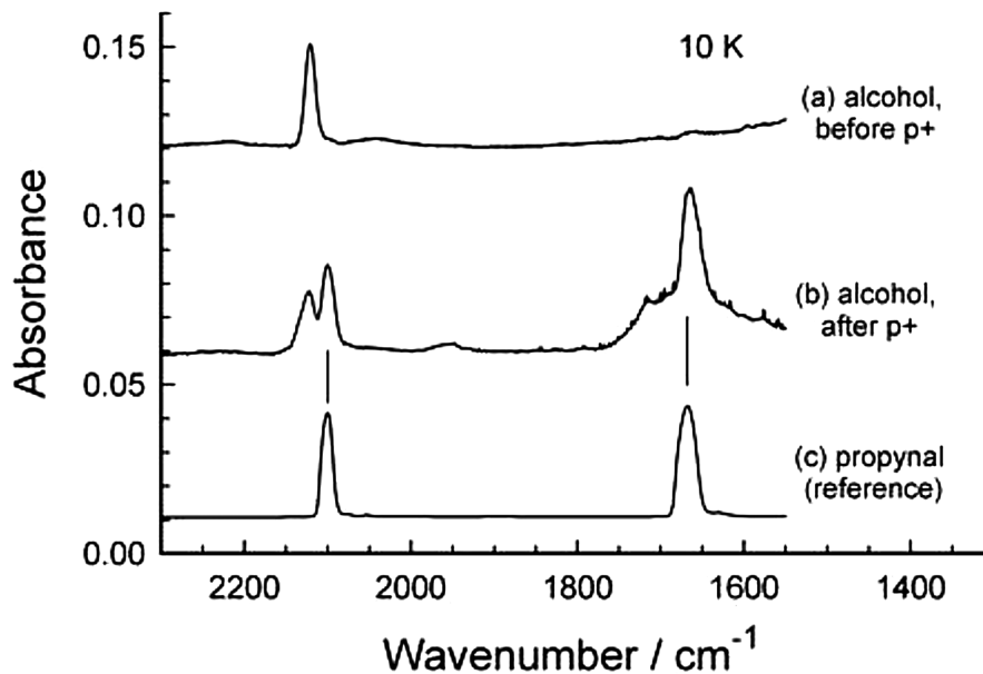
Figure 6. IR spectra of amorphous propargyl alcohol at 10 K (a) before and (b) after irradiation to a dose of \sim 3.5 \text{ eV molecule}^{-1} with 1 \text{ MeV H}^+ , compared to (c) a reference spectrum of amorphous propynal at 10 K, scaled vertically to roughly match the middle spectrum. Spectra have been offset for clarity. Small spikes in the middle spectrum between about 1800 and 1550 \text{ cm}^{-1} are due to the incomplete removal of atmospheric \text{H}_2\text{O} outside the sample chamber.
