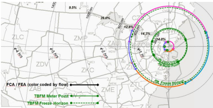
Figure 3. Integrated Demand Management Concept
