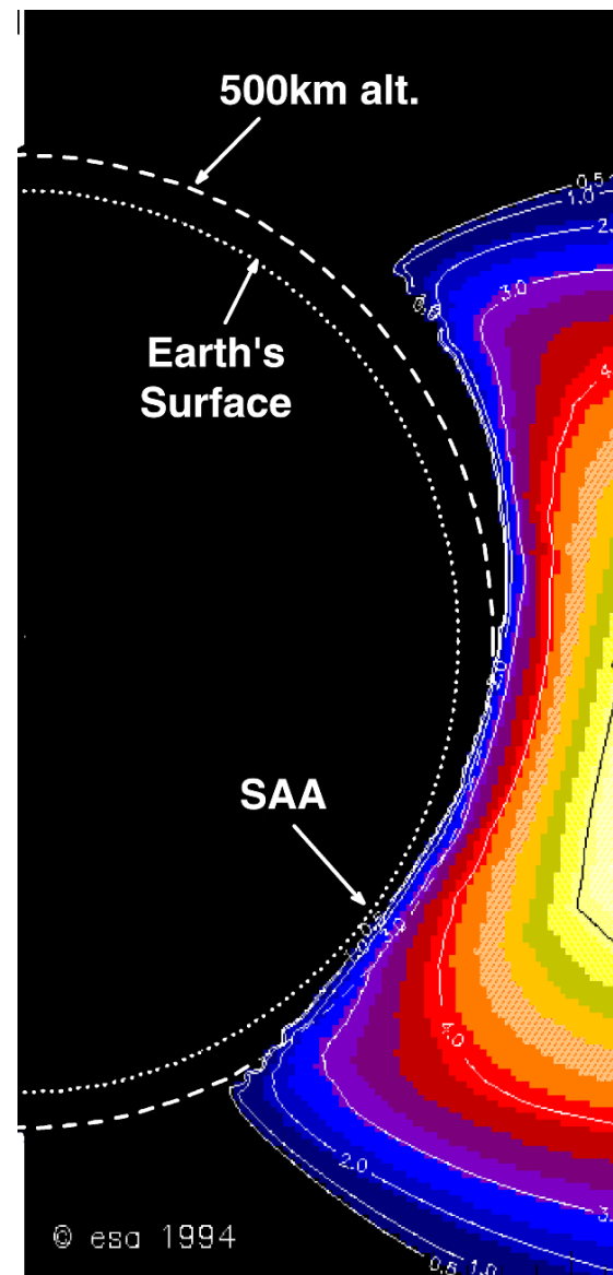
E.J. Daly et al., IEEE TNS, April 1996
