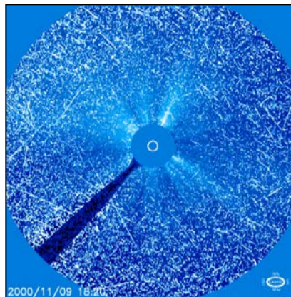
Credit: ESA and NASA (SOHO/LASCO)
