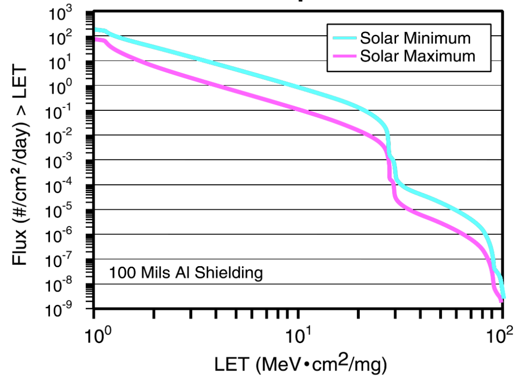
LET Spectra
