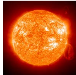
Credit: NASA (SDO)
