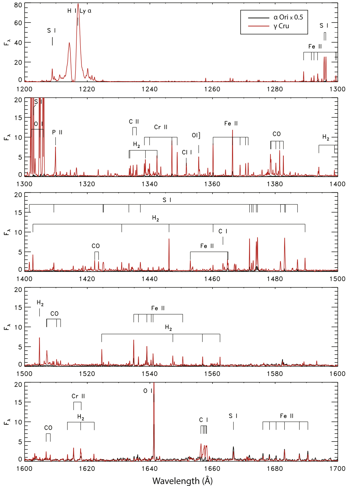
Figure 10. The 1200–1700 \text{\AA} spectral region. Selected emission lines are identified. Flux is in units of 10^{-13} \text{ erg cm}^{-2} \text{ s}^{-1} \text{ \AA}^{-1} .
