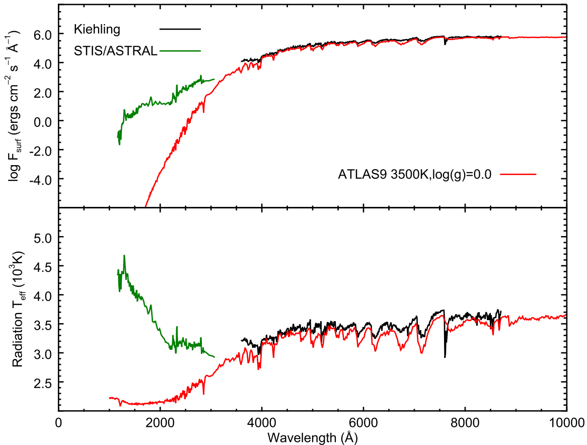
Figure 3. Top: comparison of the observed continuum surface flux distribution from \alpha Ori with a modeled Kurucz LTE ATLAS9 synthetic continuum. Observed optical data (black) are from Kiehling (1987), UV data are from HST /STIS (green), and synthetic continua were computed with a standard Kurucz model (red). Orders of magnitude separate the observed UV from the photospheric models; there is clear evidence of continuum emission from the hotter chromospheric layers. Bottom: chromospheric temperature rise implied by the observed fluxes (black and green lines) shown in a plot of the effective radiation temperature vs. wavelength. The Kurucz model temperature vs. wavelength is also shown for comparison.
