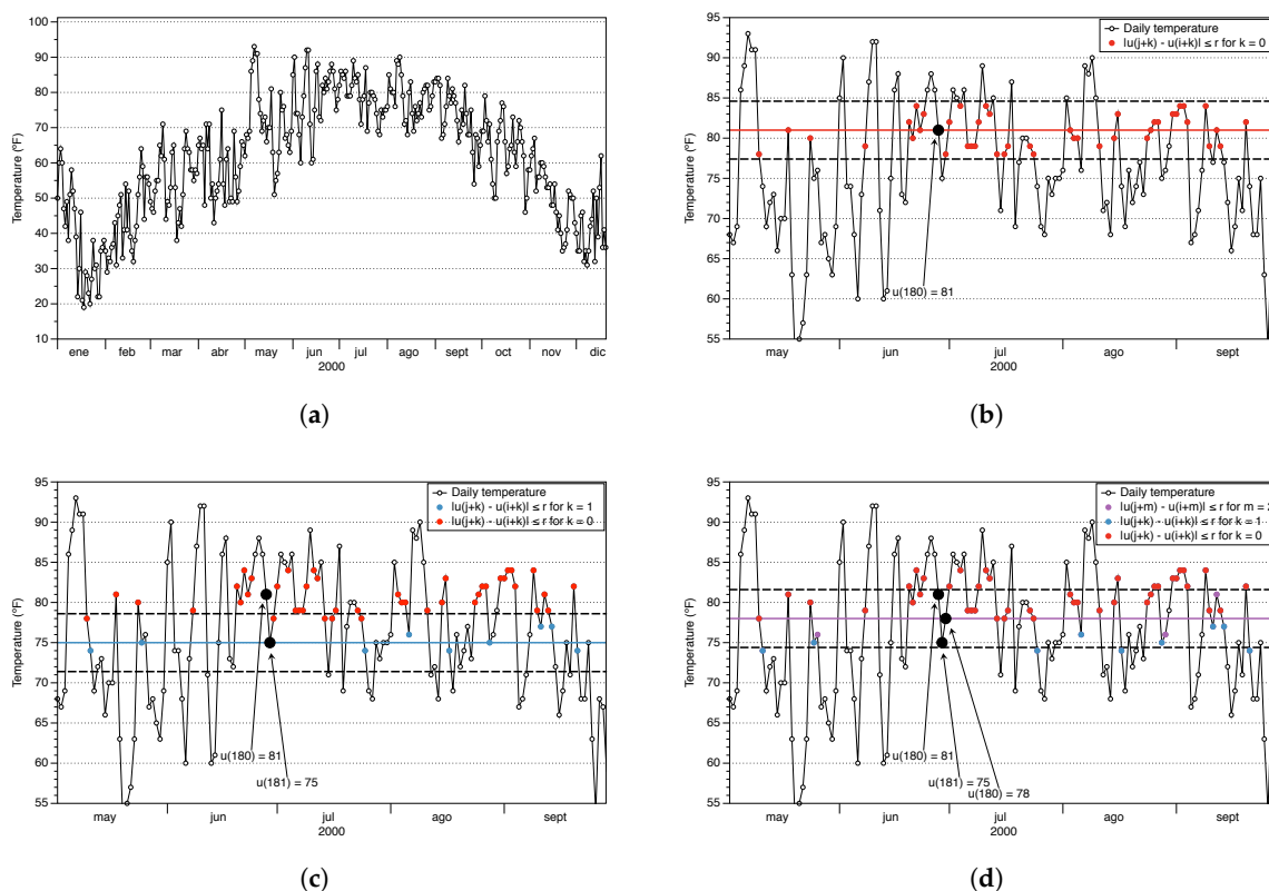
Figure 4. NYC temperatures and ApEn parameters r = 0.2\sigma and m = 2 . (a) New York City (NYC) temperature for the year 2000. (b) Red points verify that d[x(i+k), x(j+k)] \leq r for k = 0 . (c) Blue points verify that d[x(i+k), x(j+k)] \leq r for k = 1 . (d) Purple points verify that d[x(i+m), x(j+m)] \leq r for m = 2 .
