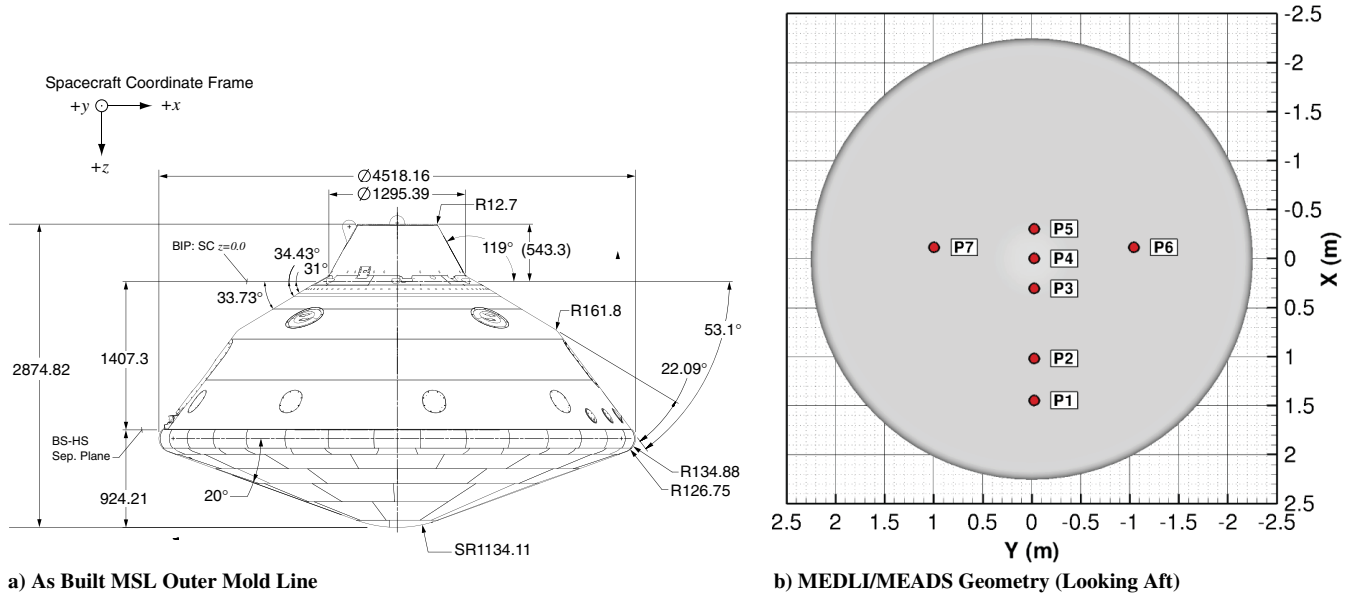
Fig. 2 Vehicle geometry.
