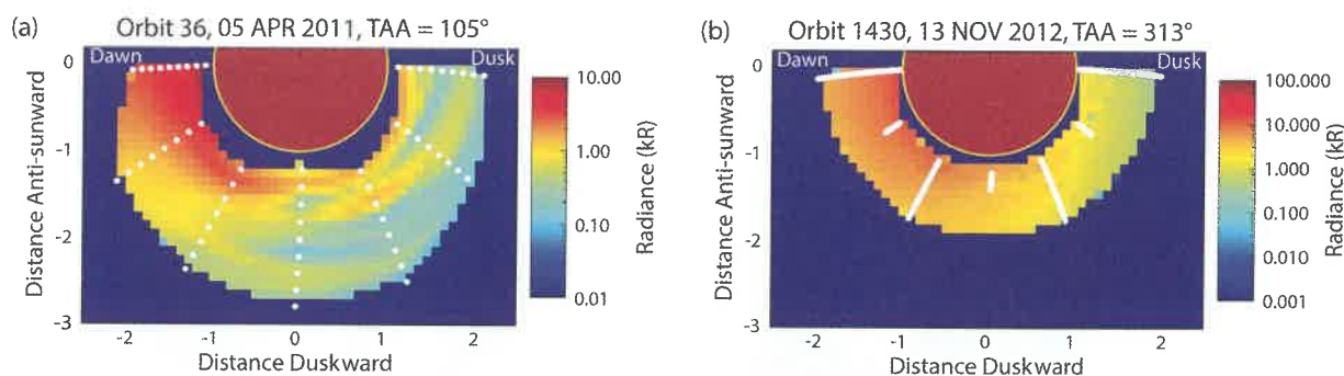
Figure 15.9. Simulated images of Ca emission in Mercury's dayside equatorial plane at two locations in Mercury's orbit were produced by interpolating between observations obtained at the white points approximately perpendicular to the plane of these images (Burger et al., 2014). In each image, dawn is to the left and the Sun is down. The white points represent positions where the UVVS line of sight crosses the equatorial plane; the altitude sampling is higher in the right panel. The images reflect large-scale local-time variations (small-scale variations in the images are not real). Although the magnitude of the emission varies with Mercury true anomaly, Ca is always brightest in the dawn hemisphere, usually, but not always, peaking at dawn.
