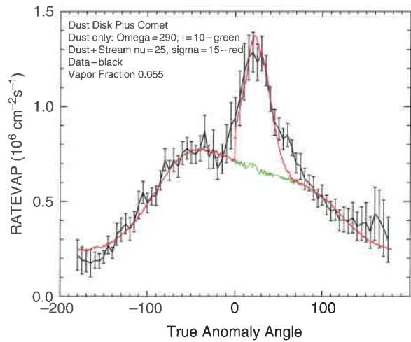
Figure 15.11. (Left) Derived source rate of Ca from the first nine Mercury years of UVVS observations plotted as a function of Mercury true anomaly angle, along with the modeled hot component of impact vaporization by the flux from interplanetary dust disk onto Mercury (green) with the addition of dust from the comet 2P/Encke centered near 25° (red) (Killen and Hahn, 2015). Away from 0–70° TAA the red line follows the dust-disk-only curve. (Right) Artist’s conception of comet dust impacting Mercury (not to scale).
