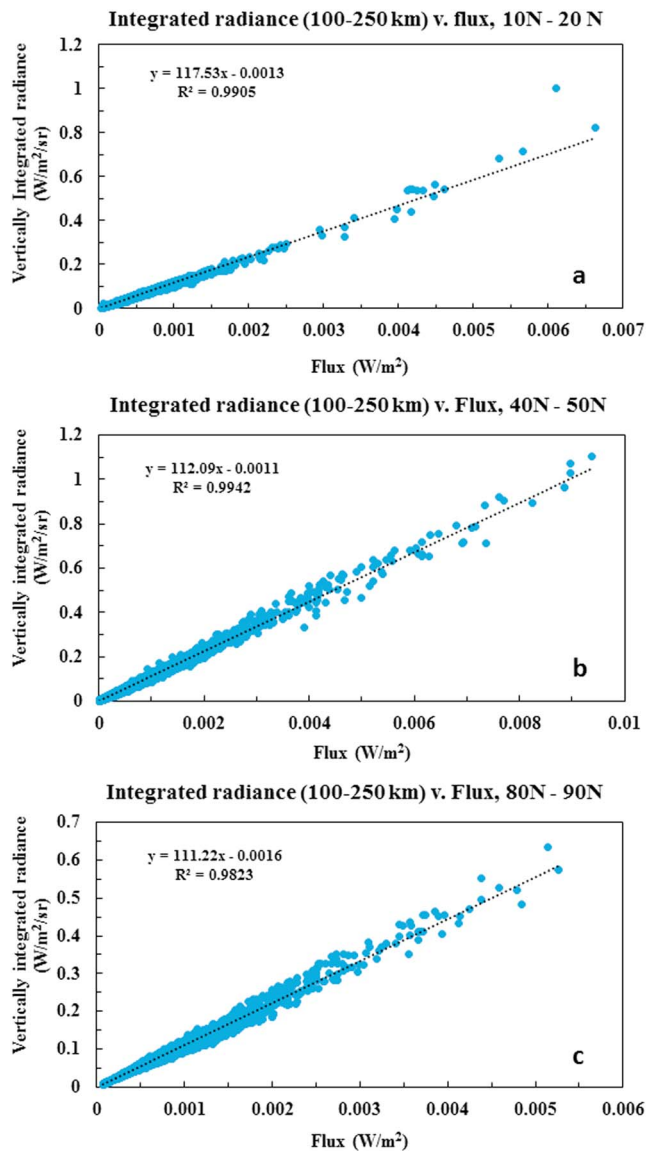
Figure 6. Sounding of the Atmosphere using Broadband Emission Radiometry (SABER) thermospheric NO flux (abscissa, \text{W/m}^2 ) versus vertically integrated SABER limb radiance (ordinate), in three different 10^\circ latitude bins, 10^\circ\text{N} – 20^\circ\text{N} (a), 40^\circ\text{N} – 50^\circ\text{N} (b), and 80^\circ\text{N} – 90^\circ\text{N} (c). These figures imply that wide field-of-view radiances are related accurately to a geophysically significant quantity, thus allowing the infrared sentinel data to serve as both a space weather forecast tool and a monitor of solar-terrestrial coupling over the long term.
