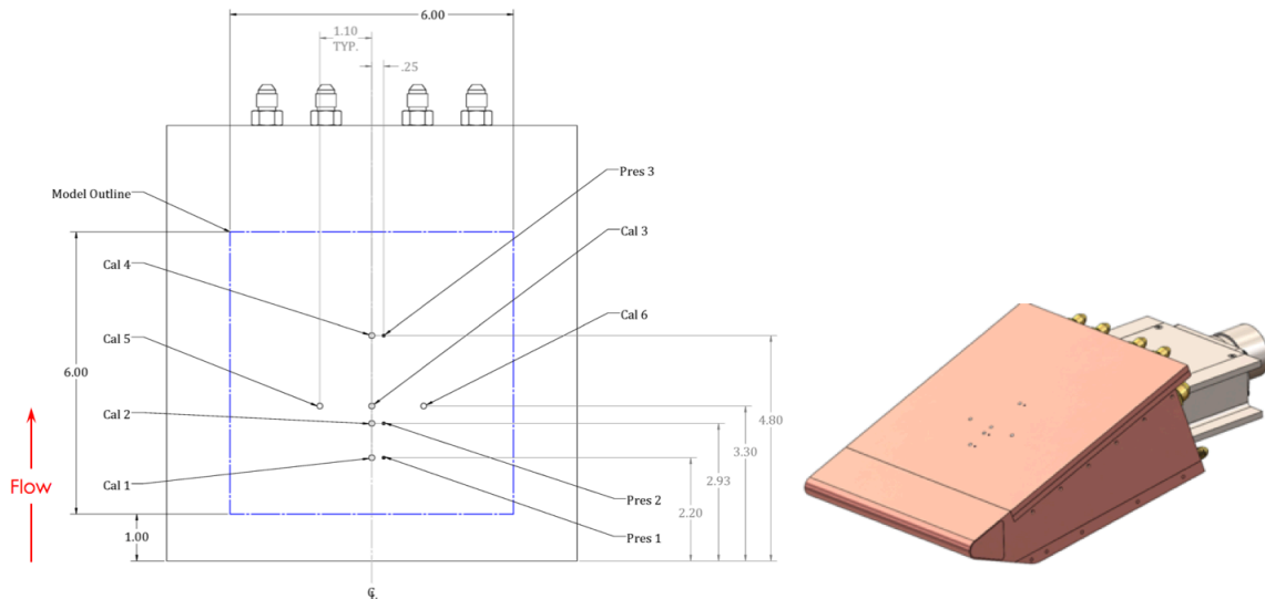
Figure 1. On left, water-cooled calibration plate drawing with dimensions in inches. Location of Gardon gages denoted by Cal , pressure transducers denoted by Pres , and laser beam target area outlined in blue. On right, assembly drawing of plate mounted onto a water-cooled wedge holder. Note that the radiative calibration plate was not instrumented with pressure sensors while the convective calibration plate did include pressure sensors.
