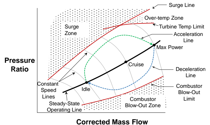
Figure 8. Compressor map indicating engine steady-state operation, transient operation, and operating limits
