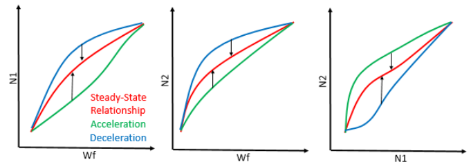
Figure 10. Schematic of the N1/N2/Wf relationship during steady-state and acceleration/deceleration transients. The black arrows indicate the desire to modify the shaft speeds during transients to operate closer to the steady-state operating line.
