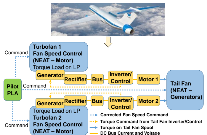
Figure 12. STARC-ABL (top) and overview diagram of STARC-ABL turbomachinery and electrical system interconnections implemented at NEAT facility (bottom)
