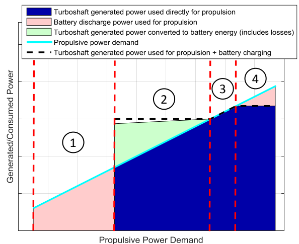
Figure 6. Notional hybrid EAP power control schedule
