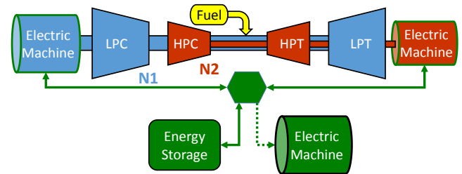
Figure 9. TEEM architecture
