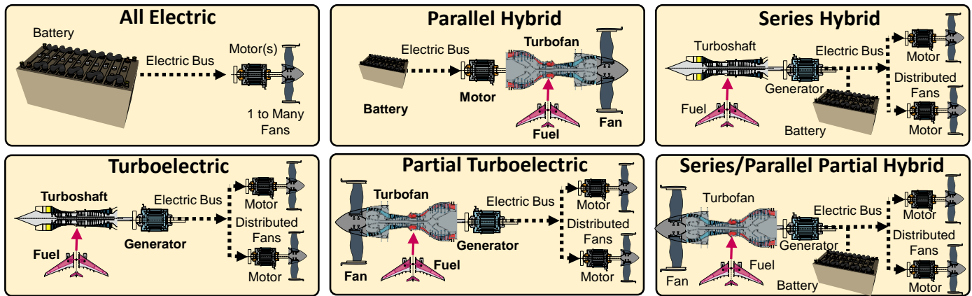
Figure 1. Electrified aircraft propulsion architectures (from Refs. [3,4])
