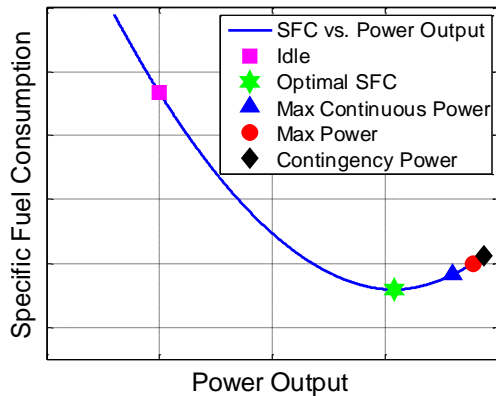
Figure 5. Notional turboshaft SFC vs. power output curve
