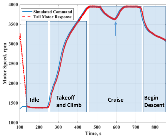
Figure 13. NEAT example flight profile tail fan spool rotational speed results with real-time turbomachinery simulation and 500 kW scaled powertrain hardware
