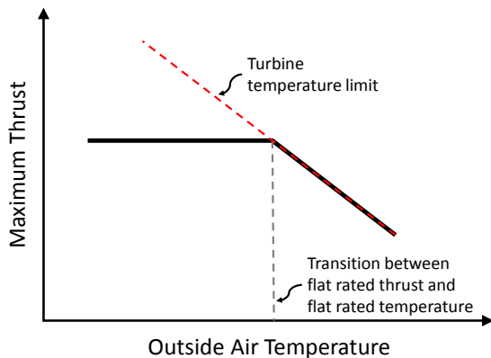
Figure 7. Engine rated thrust schedule at a fixed flight condition
