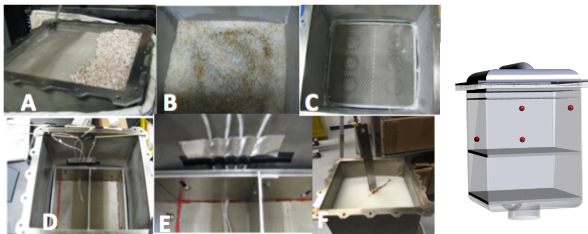
Figure 1: Pictures of the Life Test canister with (A) the Sorbead WS layer and screen, (B) a layer of the silica gel beads after bake out, (C) the middle screen surrounded by RTV sealant, (D) the new standoff installed, (E) the four RTDs to be imbedded into the sorbent layer, and (F) the silica gel layer. (right) A Solidwork diagram showing the location of the installed RTDs inside the sorbent layer (drawing per Joseph Lowman).
