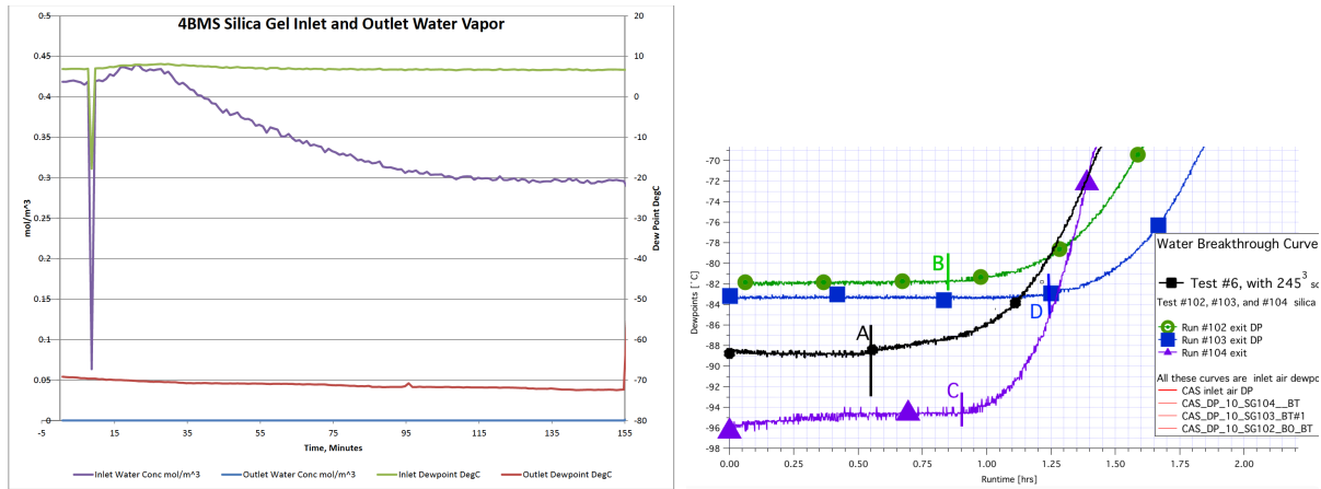
Figure 4: (left) Graphs comparing the breakthrough curves conducted at MSFC in 2006 during cyclic testing. (right) The graph showing the zoomed in section at the lower dewpoints region. Here, the different points A, B, C, and D show the different breakthrough times for the different runs.
