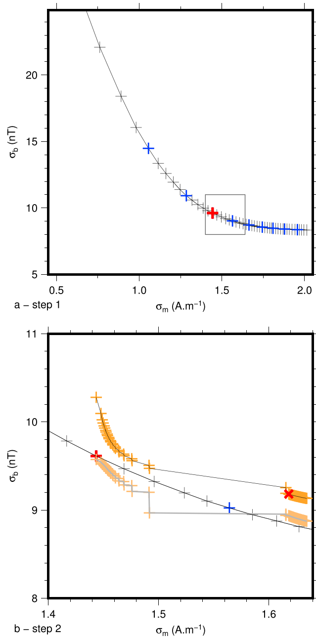
Figure D1. Evolution of the misfit \sigma_{b_i} as a function of \sigma_{m_i} . (a) First step with vector measurement only, \sigma_{b_{v_i}} . Black pluses and lines show all iterations. Blue pluses are plotted every five iterations, and the red one designs the final one. (b) Close-up on second step, when scalar measurements are added. Orange pluses show all iterations, and blue ones are plotted every five iterations. Fade symbols and line show the evolution of \sigma_{b_{v_i}} during step 2. The final model is denoted by the red cross.
