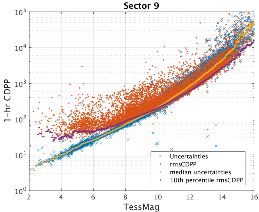
Figure 6: 1-hour CDPP. The red points are the RMS CDPP measurements for the 1996 light curves from Sector 9 plotted as a function of TESS magnitude. The blue x's are the uncertainties, scaled to 1-hour timescale. The purple curve is a moving 10th percentile of the RMS CDPP measurements, and the gold curve is a moving median of the 1-hr uncertainties.
