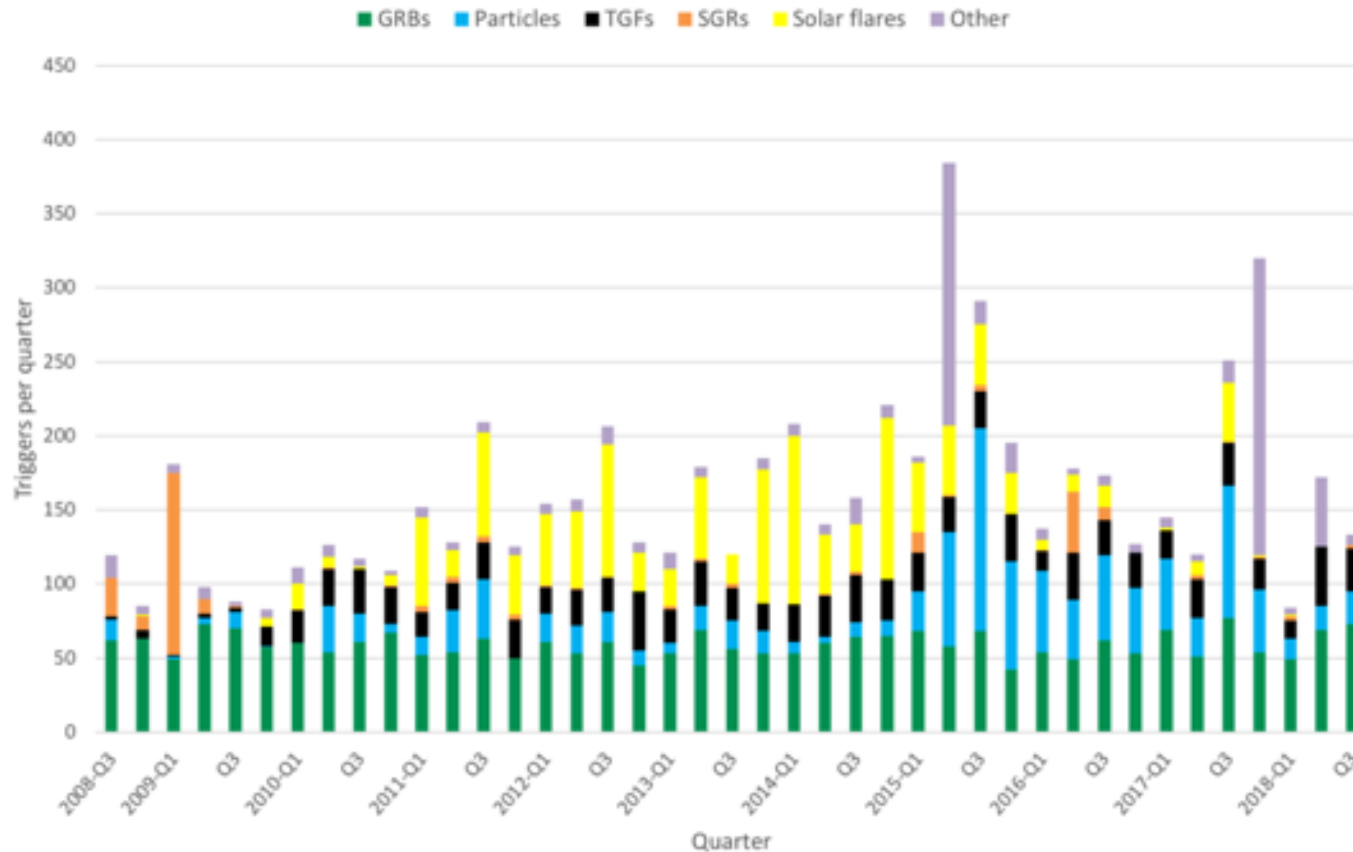
Fermi GBM Trigger History
