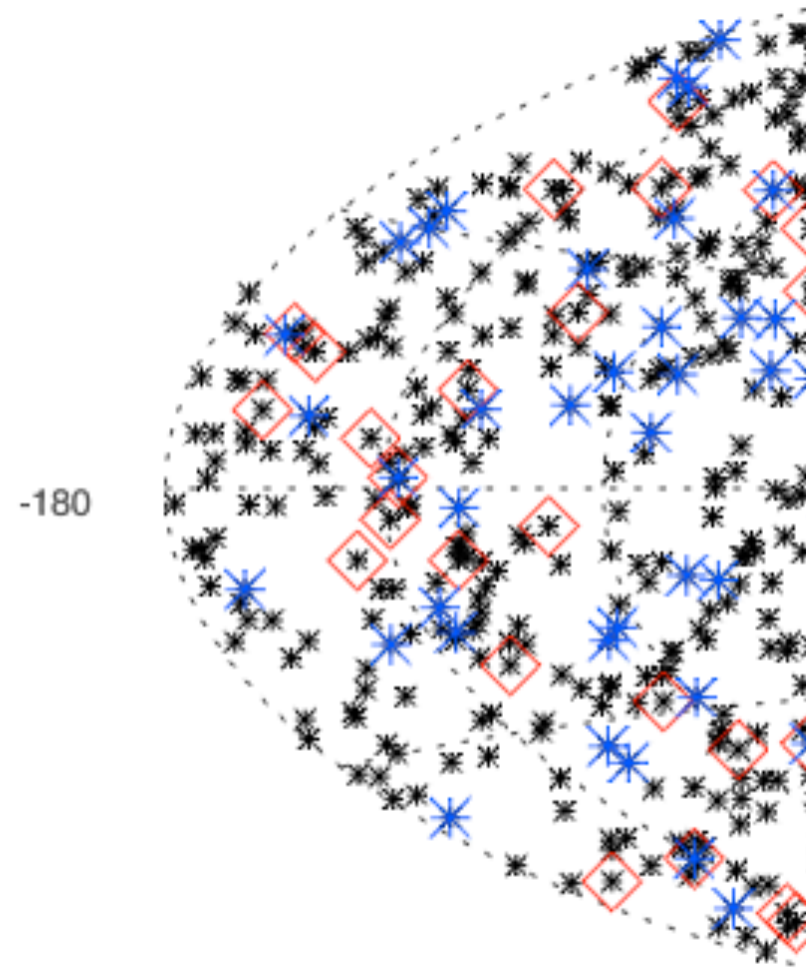
2000 GBM GRBs 266 Swift GRBs 121 LAT GRBs
