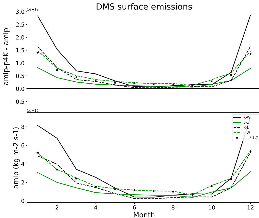
Figure 11. Seasonal cycle of dimethyl sulfide (DMS) surface emissions using different combinations of seawater concentration and emission parametrizations: Kettle-Wanninkhof (K-W), Lana-Liss (L-L), Kettle-Liss (K-L), and Lana-Wanninkhof (L-W). The 1.7 DMS scaling used in GA7.1 is shown by the L-L*1.7 stars. Regional averages between 50°S and 70°S.
