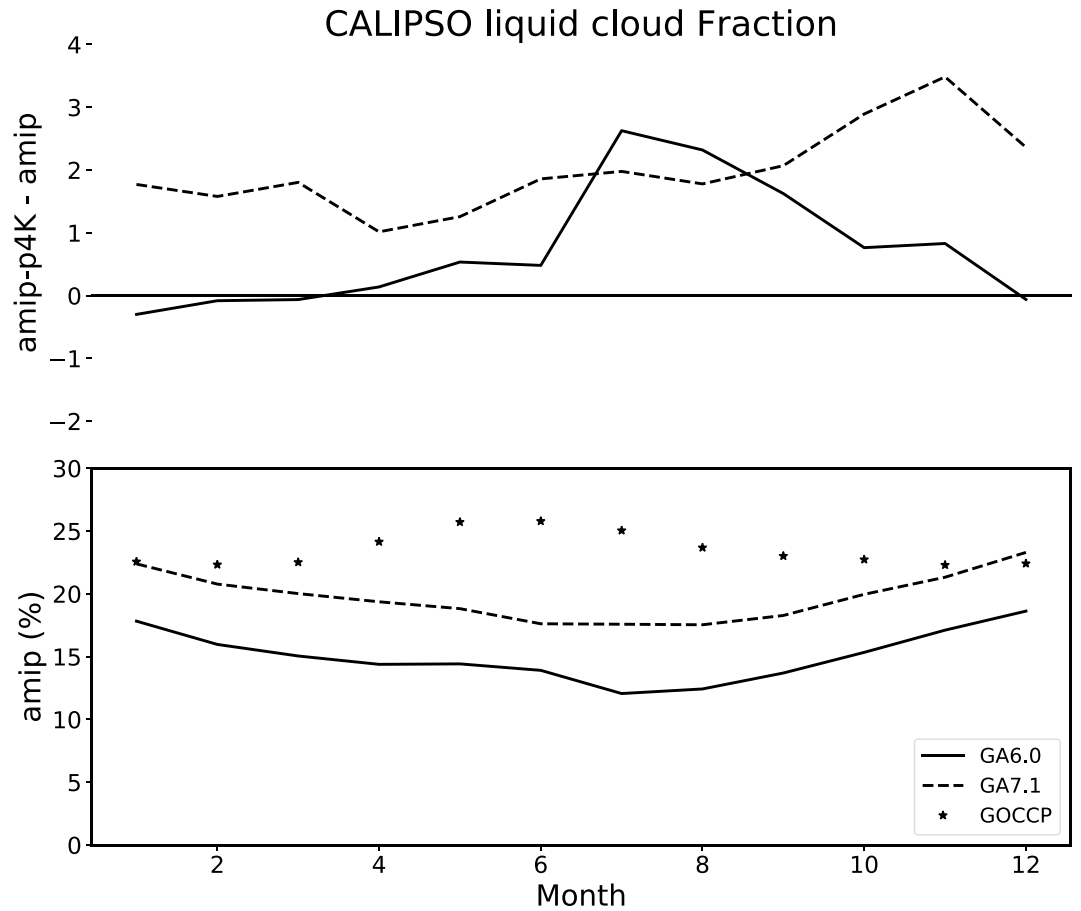
Figure 8. Seasonal cycles for COSP/CALIPSO liquid cloud fraction at 720-m altitude for the region between 50°S and 70°S. Control climatology shown in the bottom plot, and the amip-p4K minus amip response at the top. Two model configurations are shown: GA6.0 and GA7.1. GOCCP observational climatology is also displayed.
