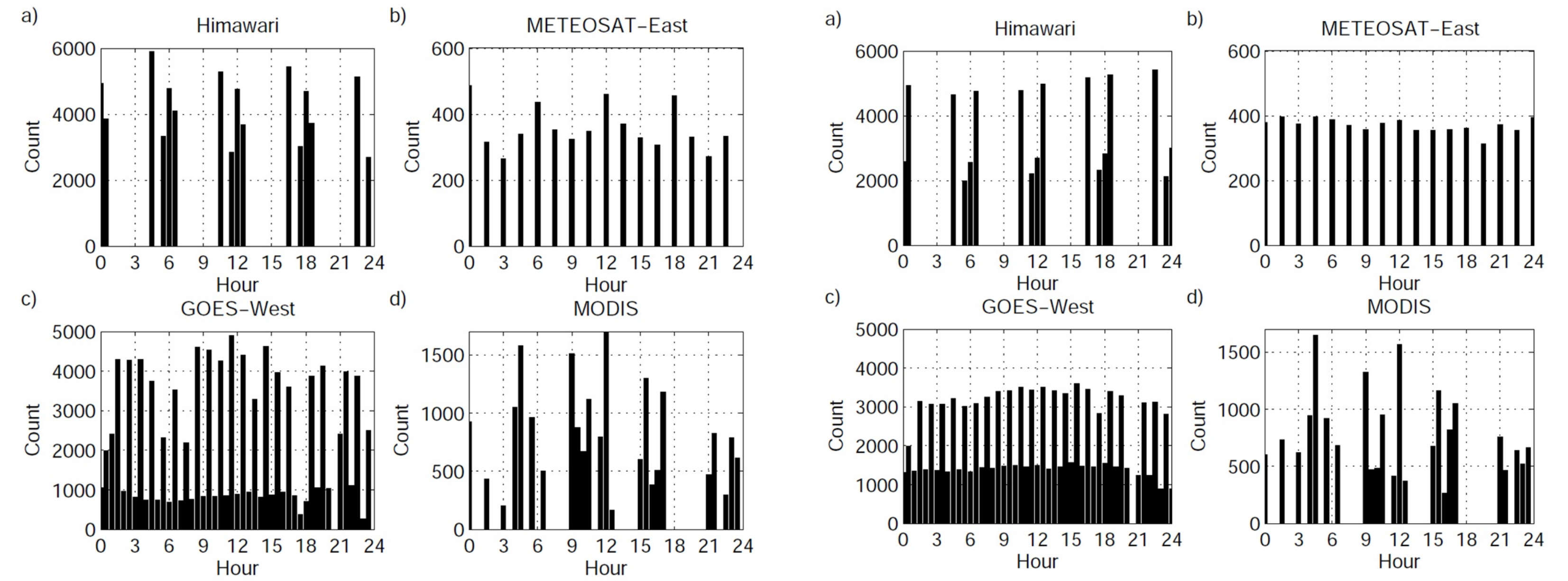
Figure 3. Numbers of locations of real (left) and simulated (right) observations within 30-min temporal bins centered at the indicated times (UTC) during 1 July (2015, left; 2006, right), produced from IR images of selected instruments.
