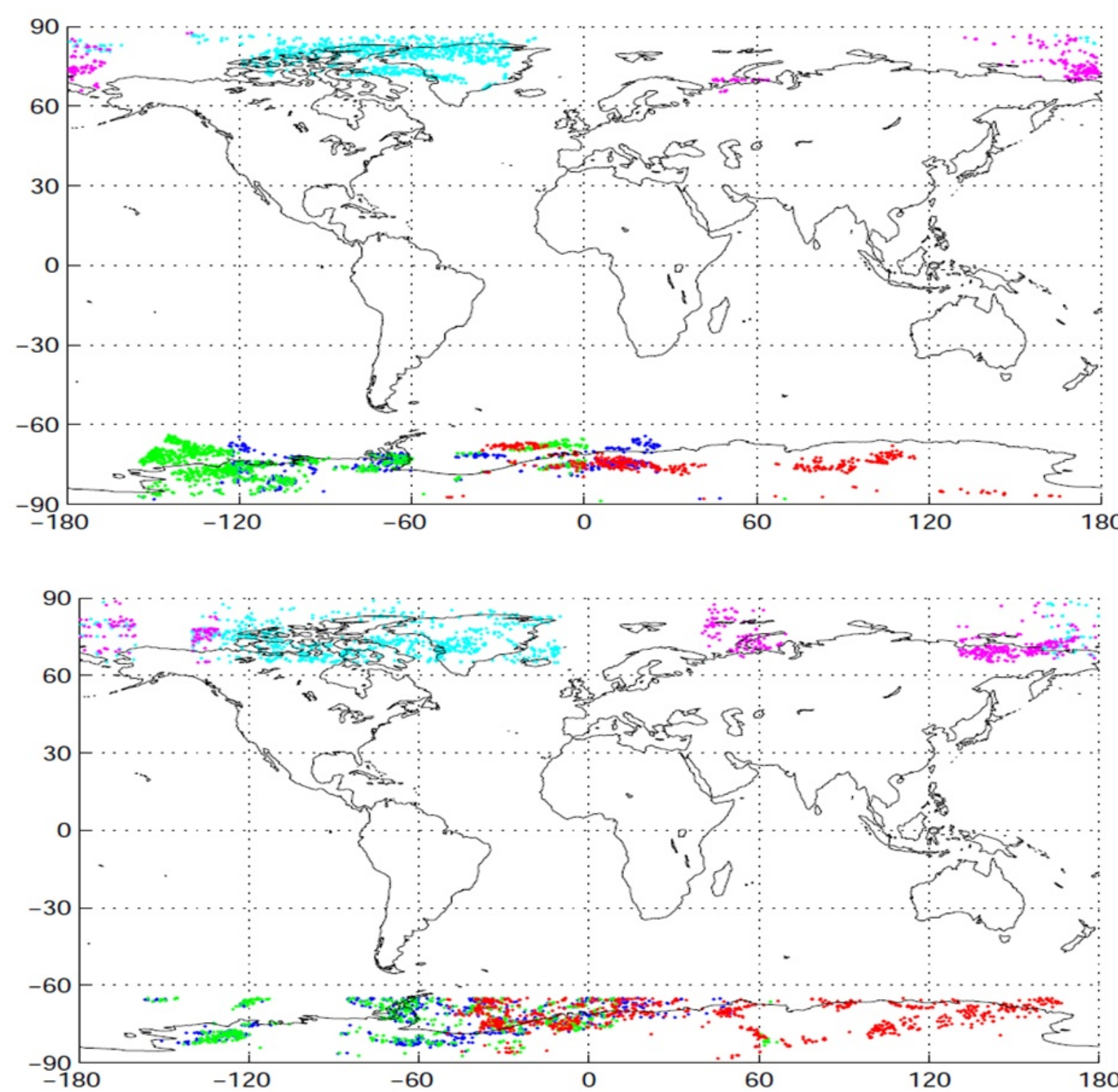
Figure 2. Locations of real (top) and simulated (bottom) MODIS AMVs assimilated at 0000 UTC 1 July (2015, top; 2006, bottom). Colors indicate observation times.
